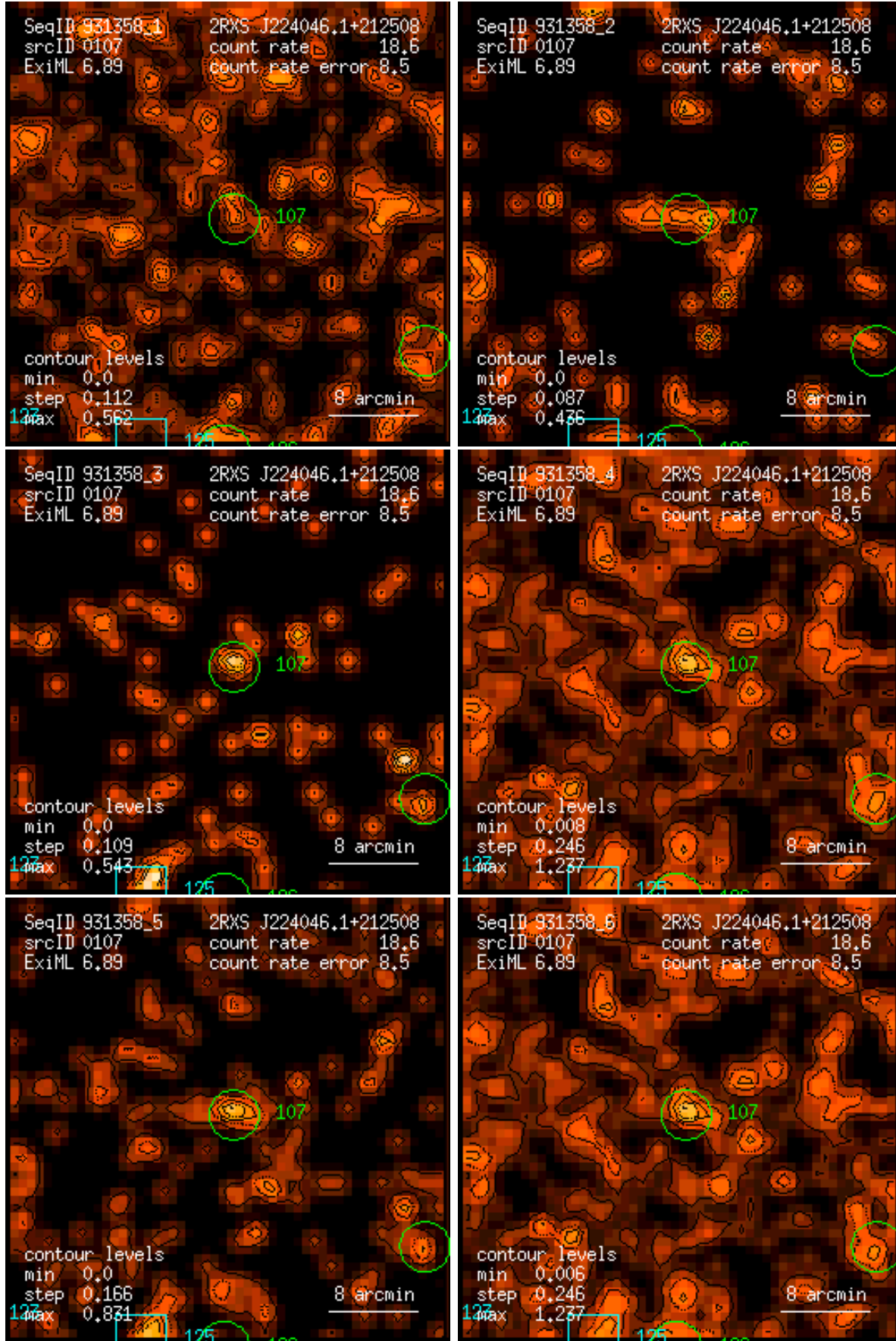
Figure 107: RASS 931358: detection 0107: band rate images, Gaussian filter: (1) PSPC channels 11 – 41, (2) 52 – 90, (3) 91 – 201, (4) 11 – 235, (5) 52 – 201, (6) 11 – 201. Broad band rates in counts/ks. Band rate contour levels in counts/ks/arcmin 2 .
