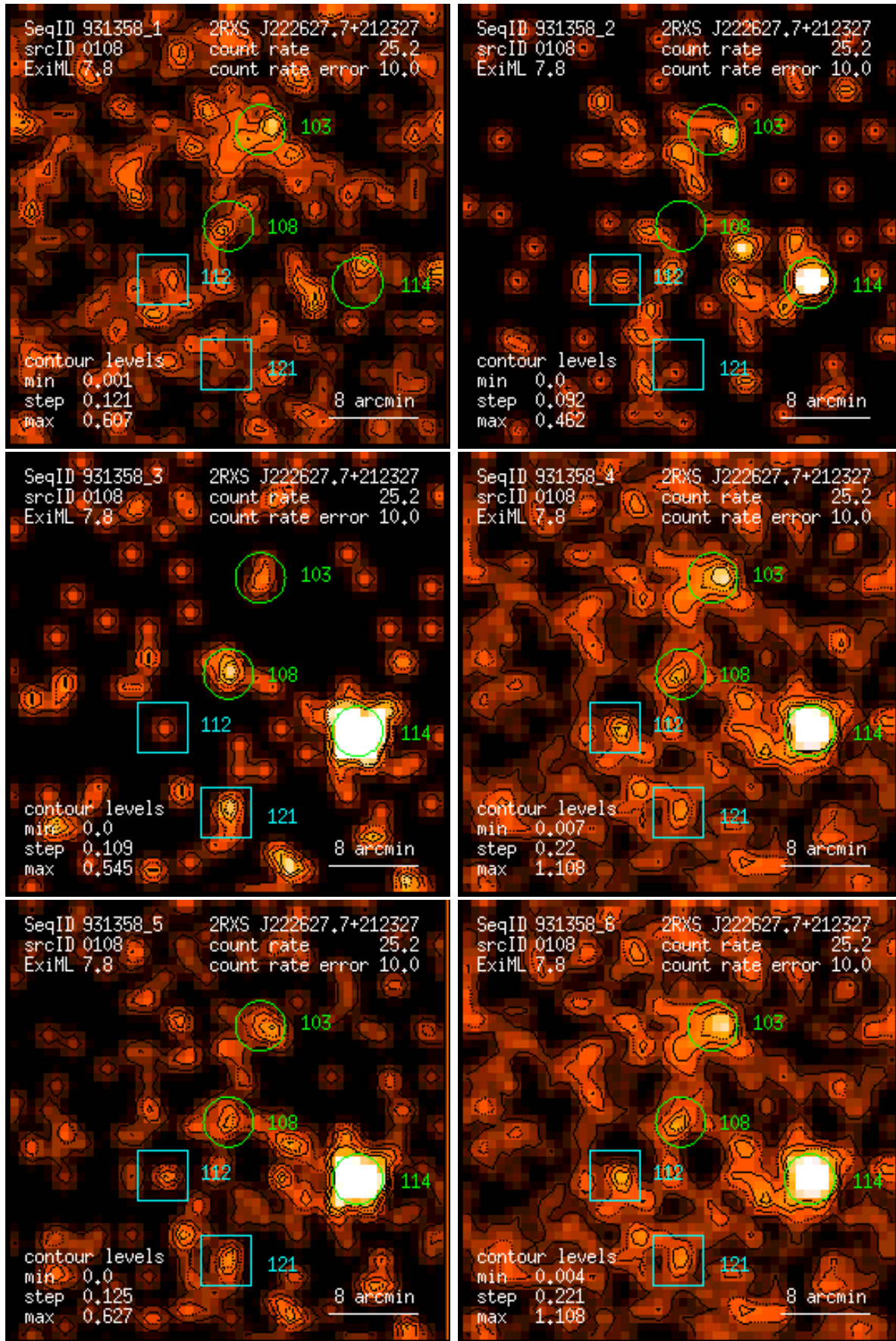
Figure 108: RASS 931358: detection 0108: band rate images, Gaussian filter: (1) PSPC channels 11 – 41, (2) 52 – 90, (3) 91 – 201, (4) 11 – 235, (5) 52 – 201, (6) 11 – 201. Broad band rates in counts/ks. Band rate contour levels in counts/ks/arcmin 2 .
