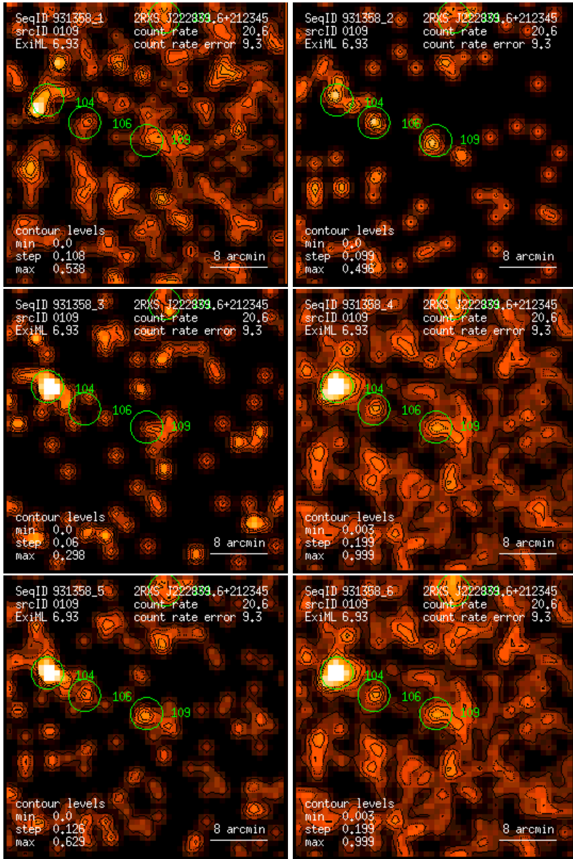
Figure 109: RASS 931358: detection 0109: band rate images, Gaussian filter: (1) PSPC channels 11 – 41, (2) 52 – 90, (3) 91 – 201, (4) 11 – 235, (5) 52 – 201, (6) 11 – 201. Broad band rates in counts/ks. Band rate contour levels in counts/ks/arcmin 2 .
