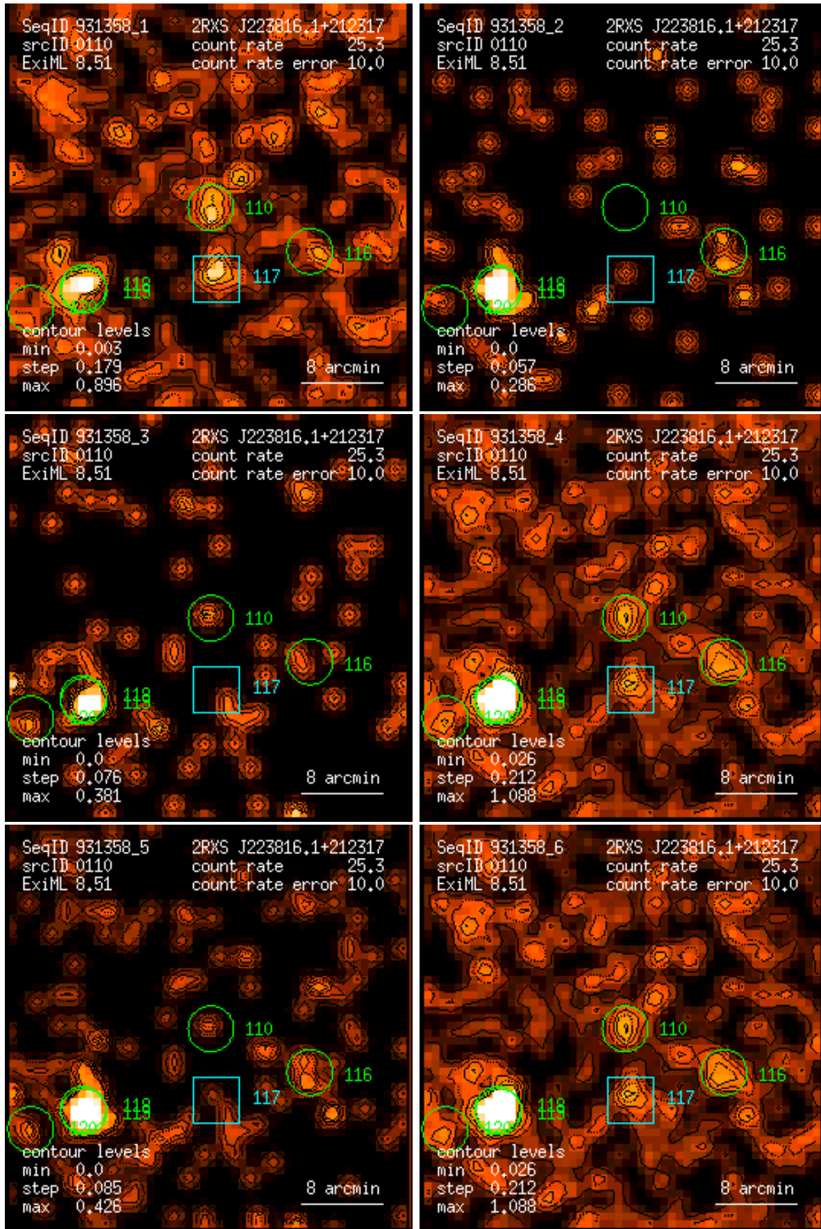
Figure 110: RASS 931358: detection 0110: band rate images, Gaussian filter: (1) PSPC channels 11 – 41, (2) 52 – 90, (3) 91 – 201, (4) 11 – 235, (5) 52 – 201, (6) 11 – 201. Broad band rates in counts/ks. Band rate contour levels in counts/ks/arcmin 2 .
