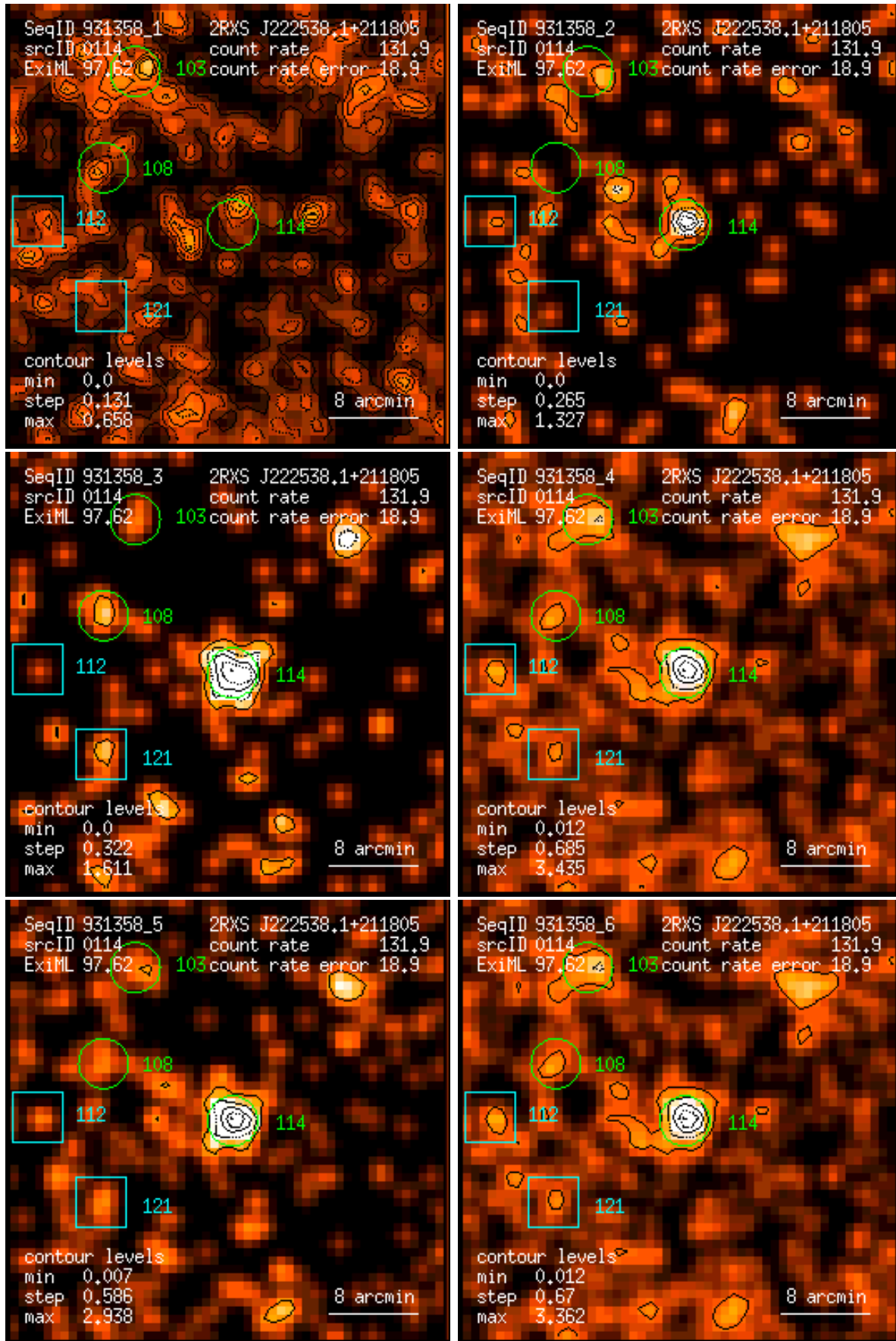
Figure 114: RASS 931358: detection 0114: band rate images, Gaussian filter: (1) PSPC channels 11 – 41, (2) 52 – 90, (3) 91 – 201, (4) 11 – 235, (5) 52 – 201, (6) 11 – 201. Broad band rates in counts/ks. Band rate contour levels in counts/ks/arcmin 2 .
