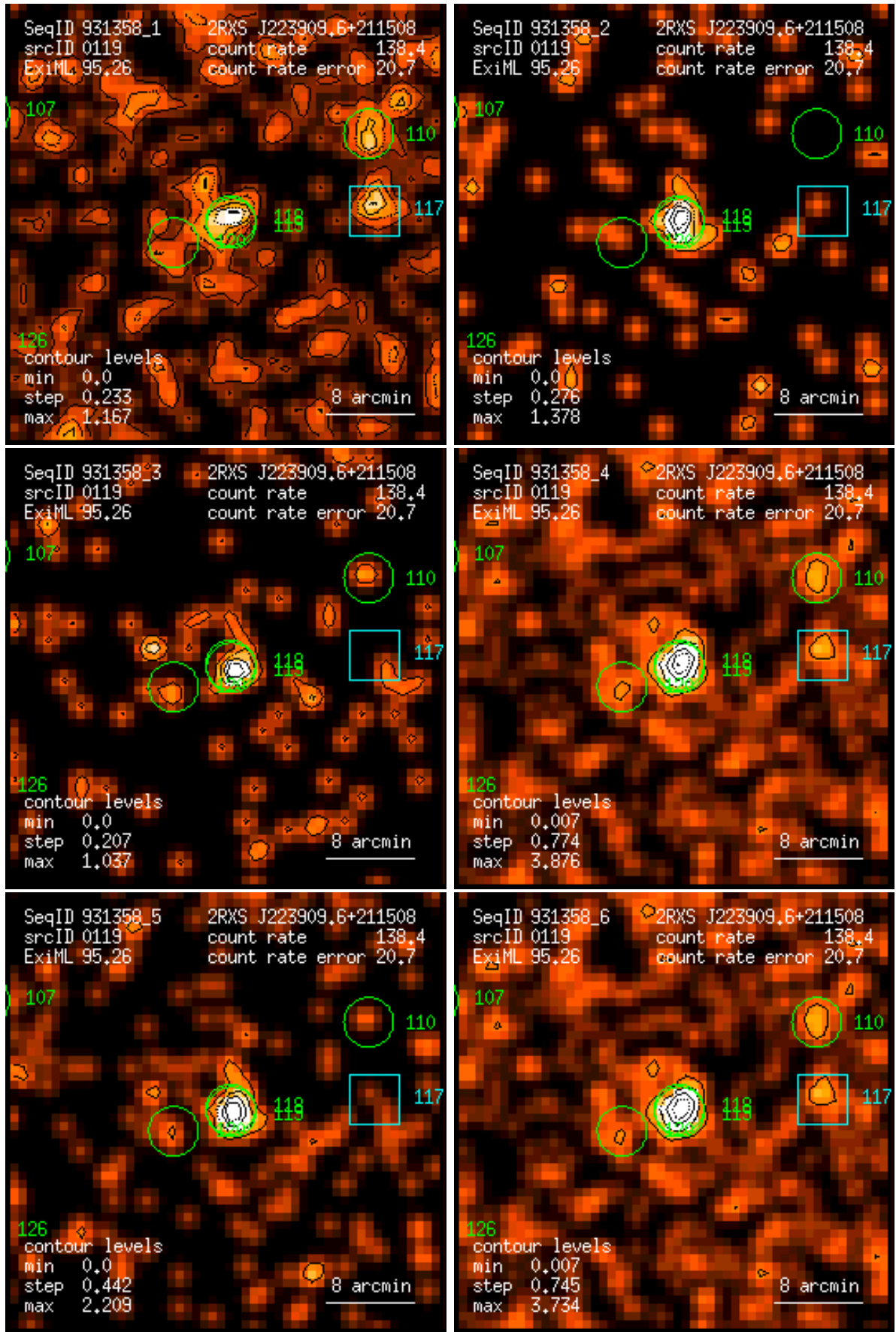
Figure 119: RASS 931358: detection 0119: band rate images, Gaussian filter: (1) PSPC channels 11 – 41, (2) 52 – 90, (3) 91 – 201, (4) 11 – 235, (5) 52 – 201, (6) 11 – 201. Broad band rates in counts/ks. Band rate contour levels in counts/ks/arcmin 2 .
