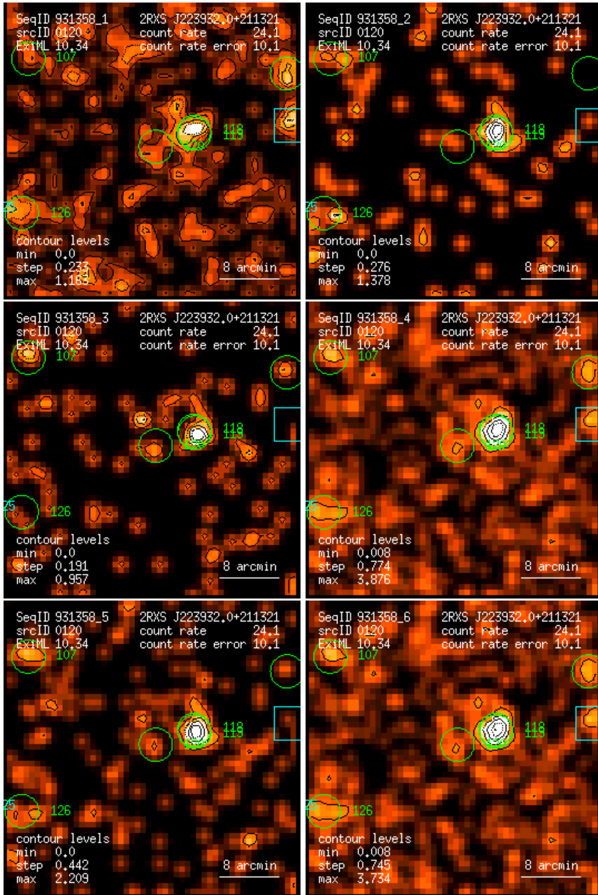
Figure 120: RASS 931358: detection 0120: band rate images, Gaussian filter: (1) PSPC channels 11 – 41, (2) 52 – 90, (3) 91 – 201, (4) 11 – 235, (5) 52 – 201, (6) 11 – 201. Broad band rates in counts/ks. Band rate contour levels in counts/ks/arcmin 2 .
