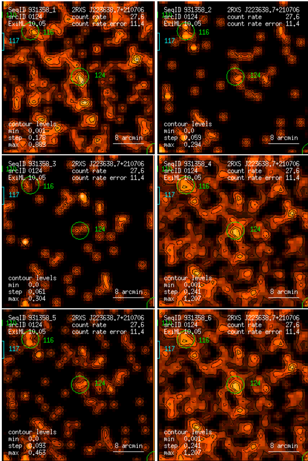
Figure 124: RASS 931358: detection 0124: band rate images, Gaussian filter: (1) PSPC channels 11 – 41, (2) 52 – 90, (3) 91 – 201, (4) 11 – 235, (5) 52 – 201, (6) 11 – 201. Broad band rates in counts/ks. Band rate contour levels in counts/ks/arcmin 2 .
