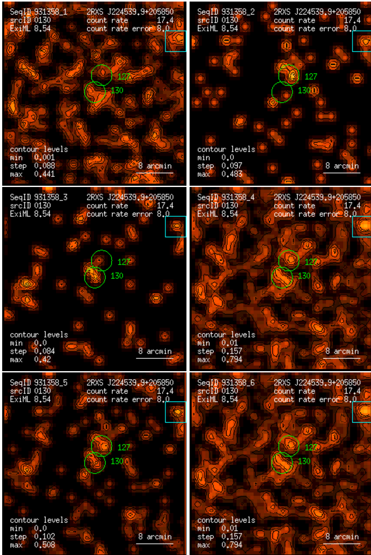
Figure 130: RASS 931358: detection 0130: band rate images, Gaussian filter: (1) PSPPC channels 11 – 41, (2) 52 – 90, (3) 91 – 201, (4) 11 – 235, (5) 52 – 201, (6) 11 – 201. Broad band rates in counts/ks. Band rate contour levels in counts/ks/arcmin 2 .
