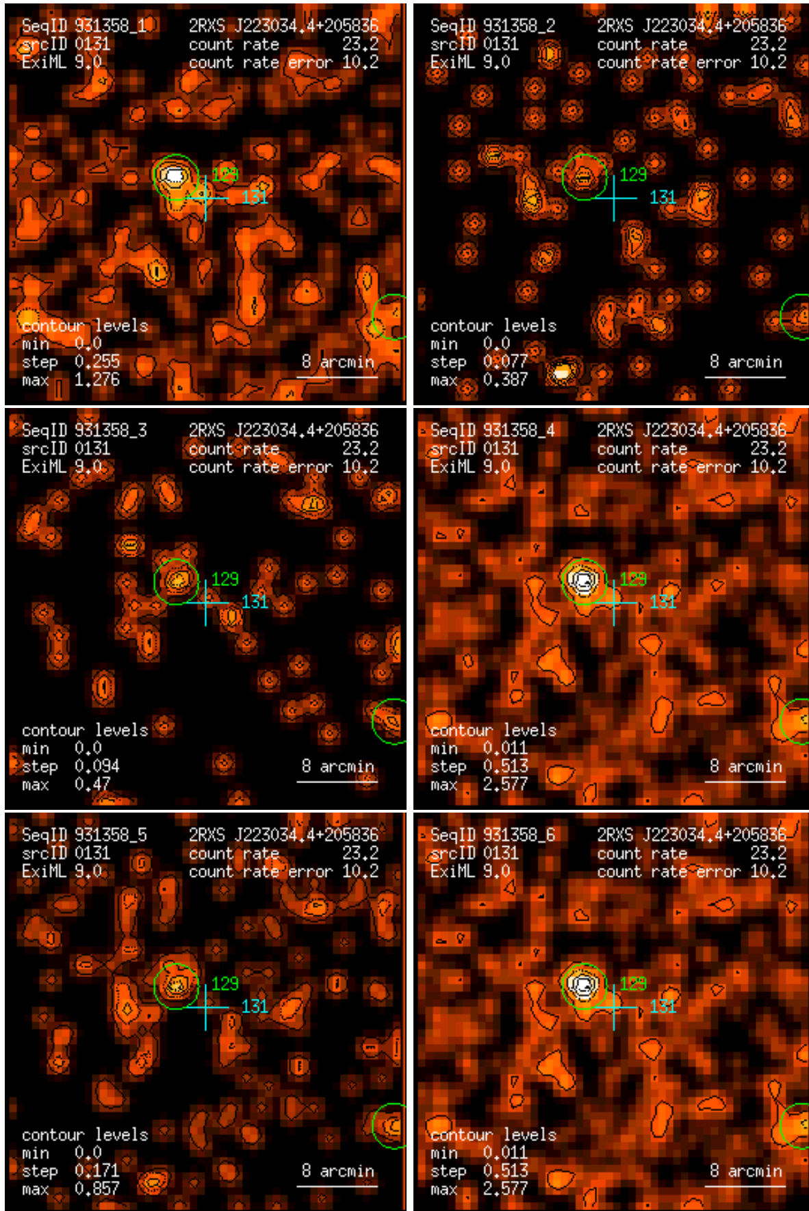
Figure 131: RASS 931358: detection 0131: band rate images, Gaussian filter: (1) PSPC channels 11 – 41, (2) 52 – 90, (3) 91 – 201, (4) 11 – 235, (5) 52 – 201, (6) 11 – 201. Broad band rates in counts/ks. Band rate contour levels in counts/ks/arcmin 2 .
