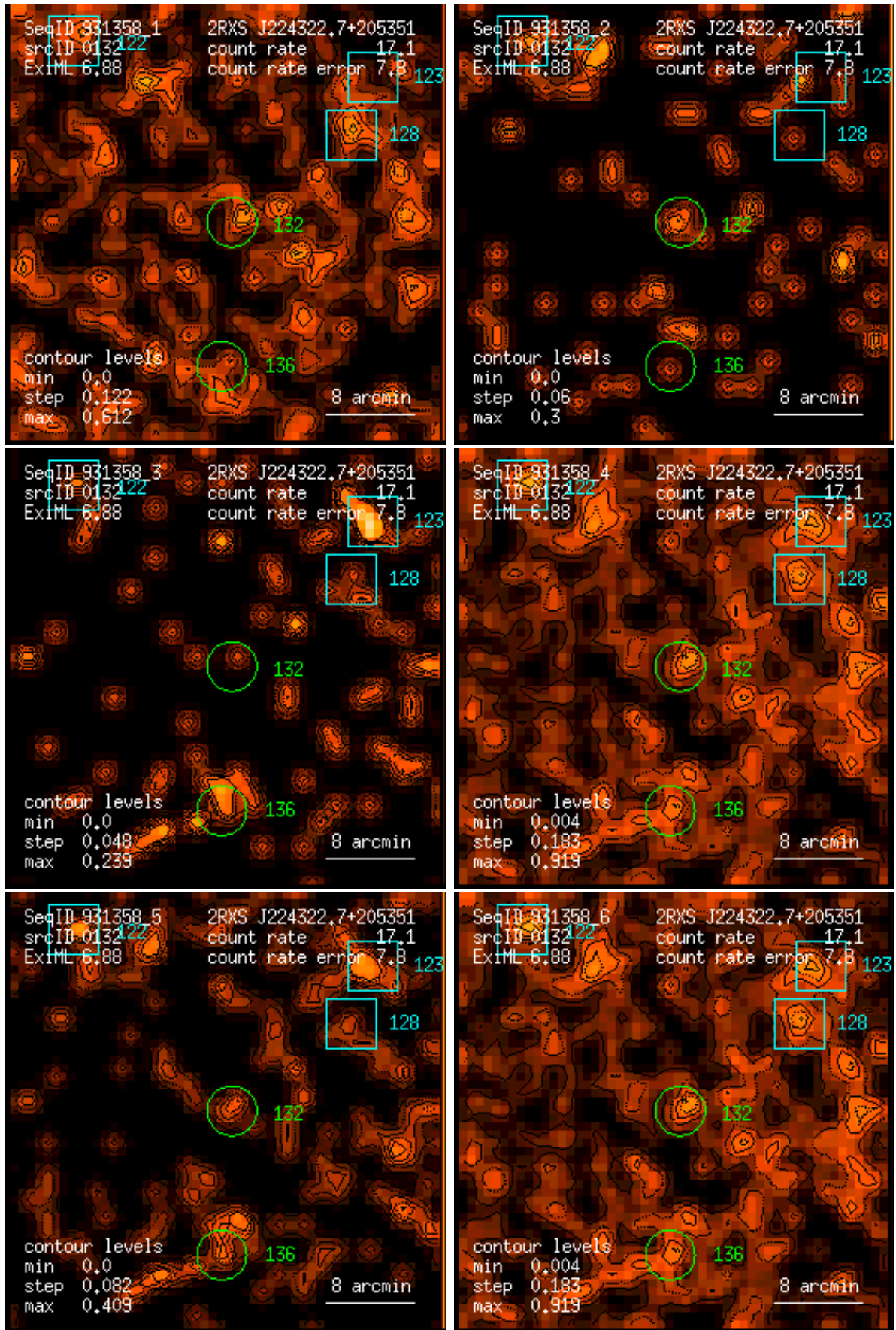
Figure 132: RASS 931358: detection 0132: band rate images, Gaussian filter: (1) PSPC channels 11 – 41, (2) 52 – 90, (3) 91 – 201, (4) 11 – 235, (5) 52 – 201, (6) 11 – 201. Broad band rates in counts/ks. Band rate contour levels in counts/ks/arcmin 2 .
