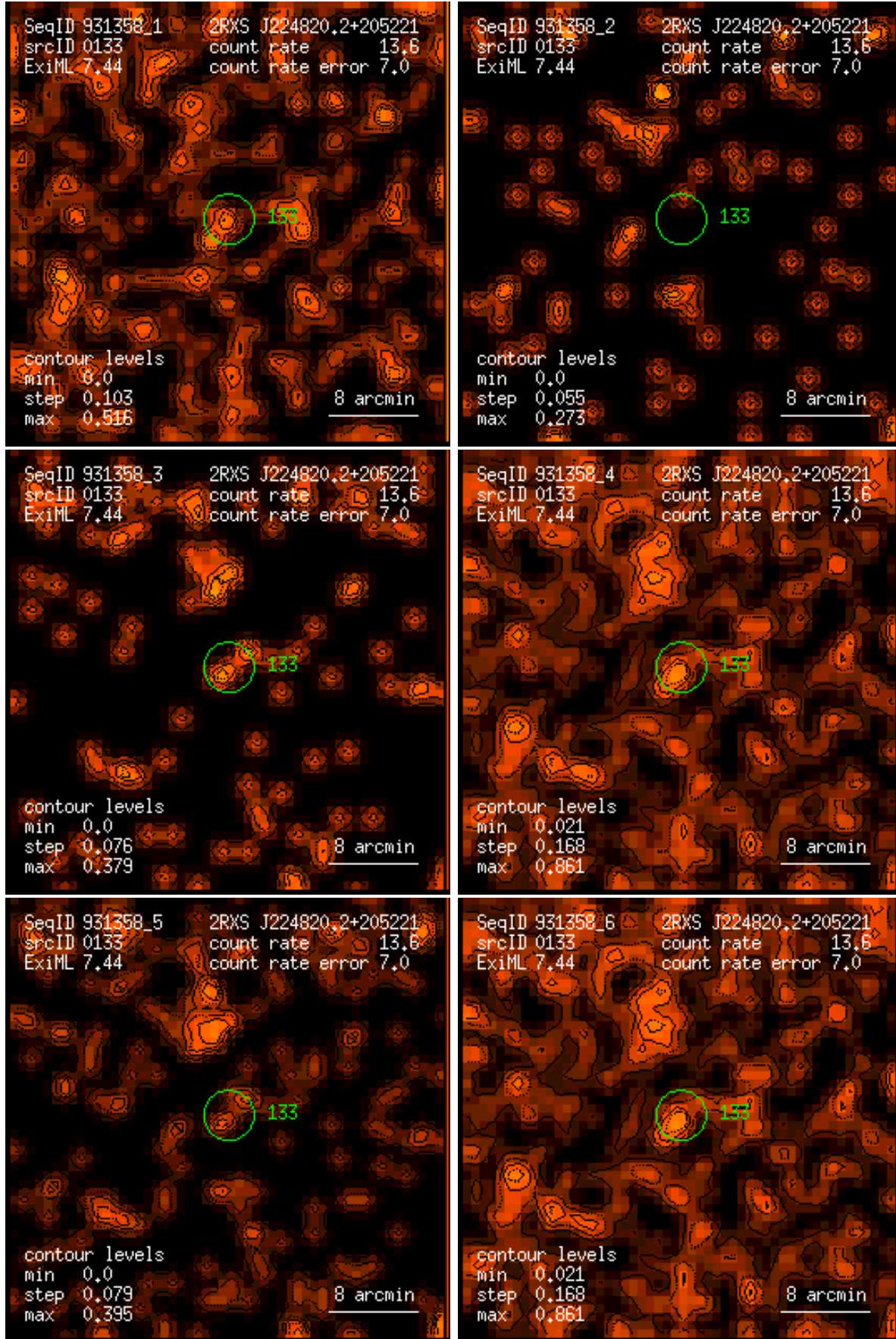
Figure 133: RASS 931358: detection 0133: band rate images, Gaussian filter: (1) PSPC channels 11 – 41, (2) 52 – 90, (3) 91 – 201, (4) 11 – 235, (5) 52 – 201, (6) 11 – 201. Broad band rates in counts/ks. Band rate contour levels in counts/ks/arcmin 2 .
