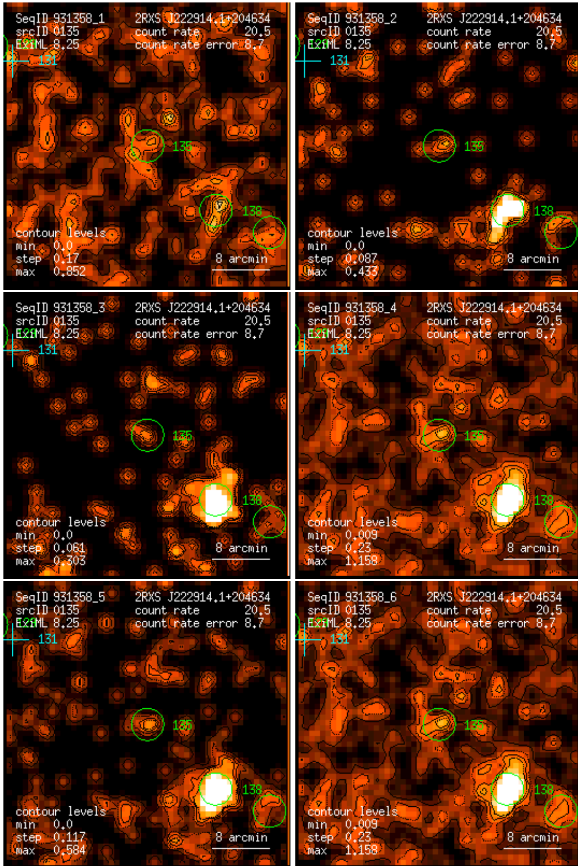
Figure 135: RASS 931358: detection 0135: band rate images, Gaussian filter: (1) PSPC channels 11 – 41, (2) 52 – 90, (3) 91 – 201, (4) 11 – 235, (5) 52 – 201, (6) 11 – 201. Broad band rates in counts/ks. Band rate contour levels in counts/ks/arcmin 2 .
