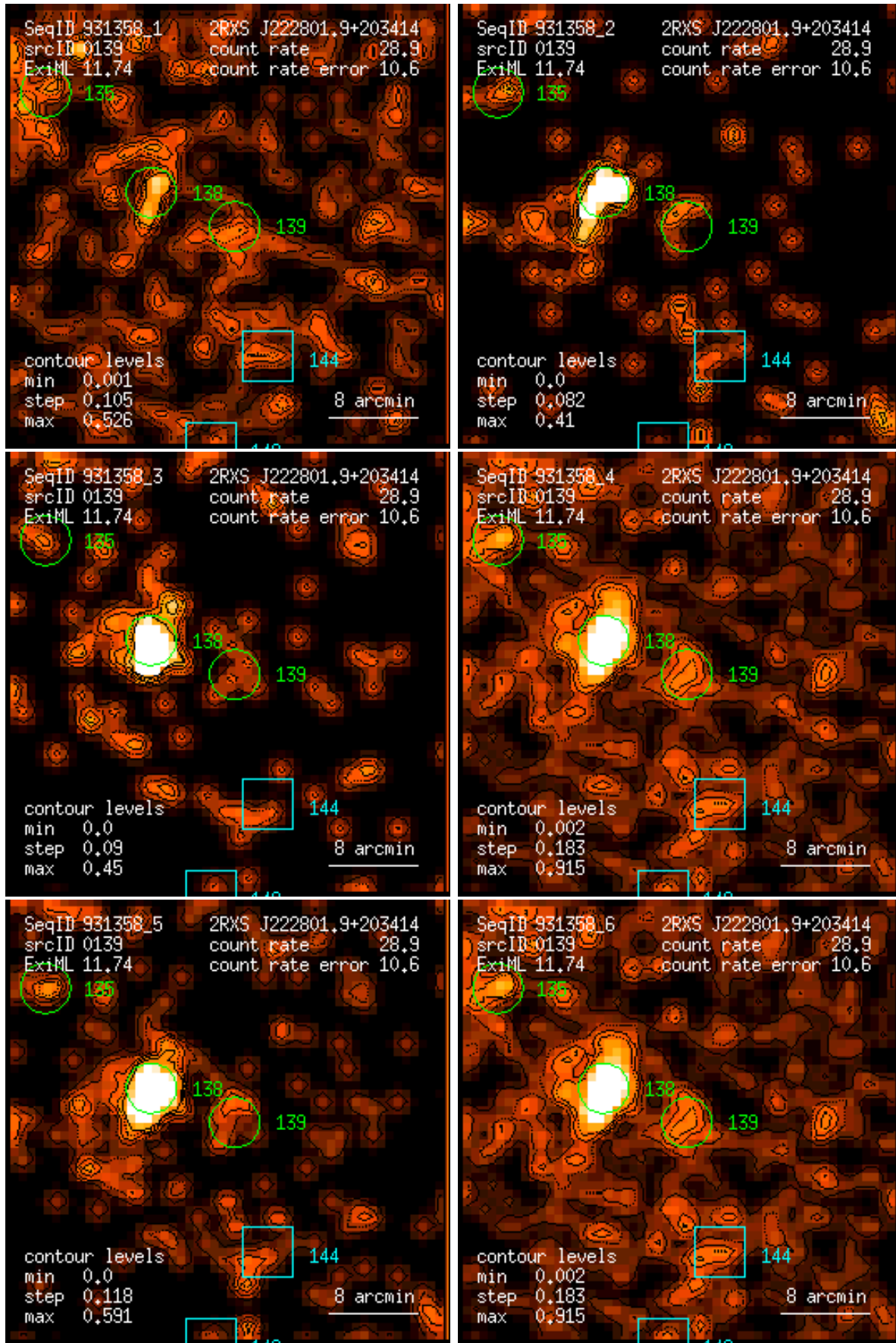
Figure 139: RASS 931358: detection 0139: band rate images, Gaussian filter: (1) PSPC channels 11 – 41, (2) 52 – 90, (3) 91 – 201, (4) 11 – 235, (5) 52 – 201, (6) 11 – 201. Broad band rates in counts/ks. Band rate contour levels in counts/ks/arcmin 2 .
