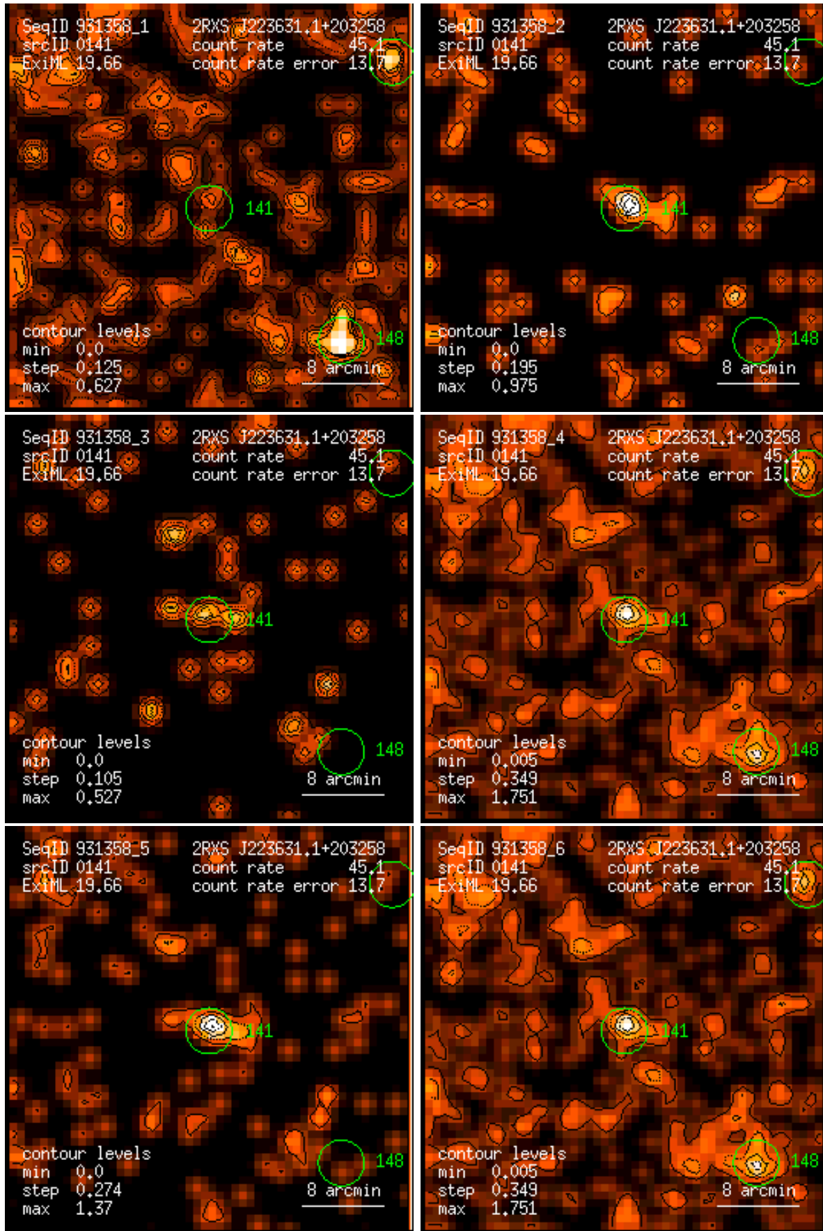
Figure 141: RASS 931358: detection 0141: band rate images, Gaussian filter: (1) PSPC channels 11 – 41, (2) 52 – 90, (3) 91 – 201, (4) 11 – 235, (5) 52 – 201, (6) 11 – 201. Broad band rates in counts/ks. Band rate contour levels in counts/ks/arcmin 2 .
