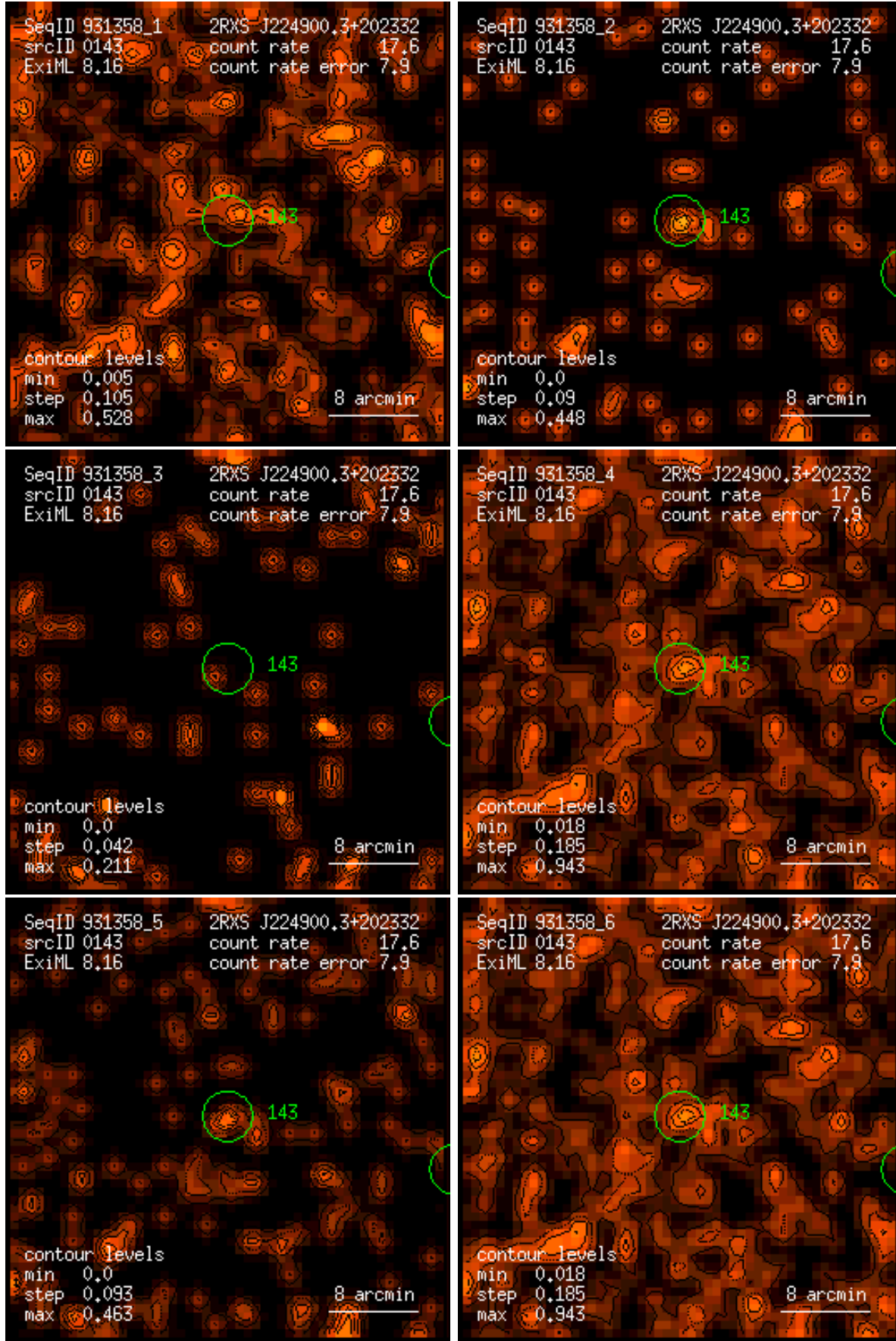
Figure 143: RASS 931358: detection 0143: band rate images, Gaussian filter: (1) PSPC channels 11 – 41, (2) 52 – 90, (3) 91 – 201, (4) 11 – 235, (5) 52 – 201, (6) 11 – 201. Broad band rates in counts/ks. Band rate contour levels in counts/ks/arcmin 2 .
