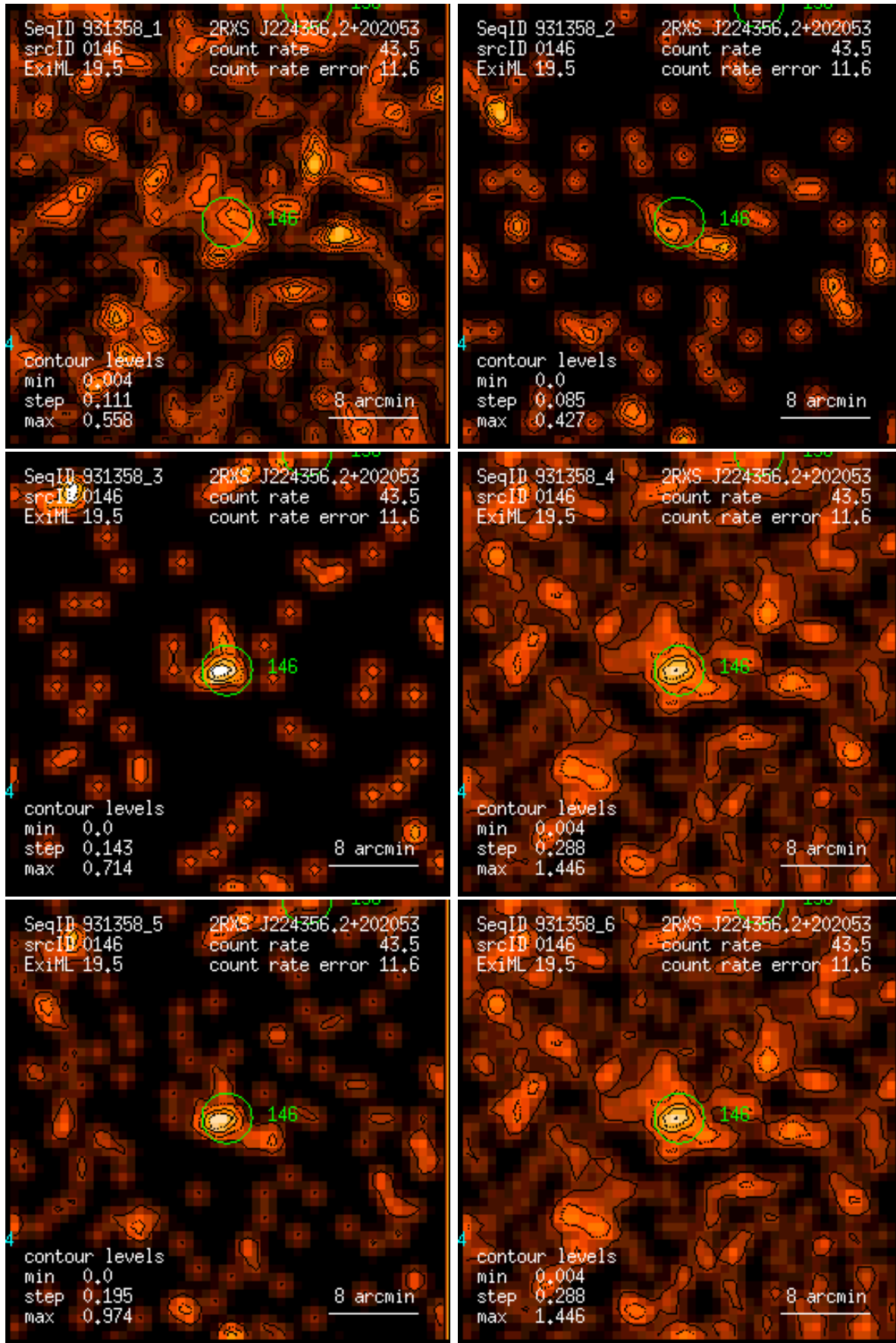
Figure 146: RASS 931358: detection 0146: band rate images, Gaussian filter: (1) PSPC channels 11 – 41, (2) 52 – 90, (3) 91 – 201, (4) 11 – 235, (5) 52 – 201, (6) 11 – 201. Broad band rates in counts/ks. Band rate contour levels in counts/ks/arcmin 2 .
