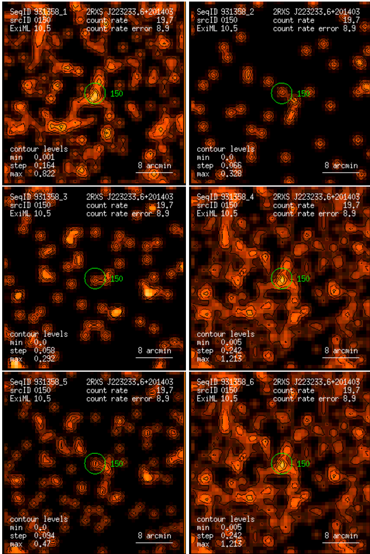
Figure 150: RASS 931358: detection 0150: band rate images, Gaussian filter: (1) PSPC channels 11 – 41, (2) 52 – 90, (3) 91 – 201, (4) 11 – 235, (5) 52 – 201, (6) 11 – 201. Broad band rates in counts/ks. Band rate contour levels in counts/ks/arcmin 2 .
