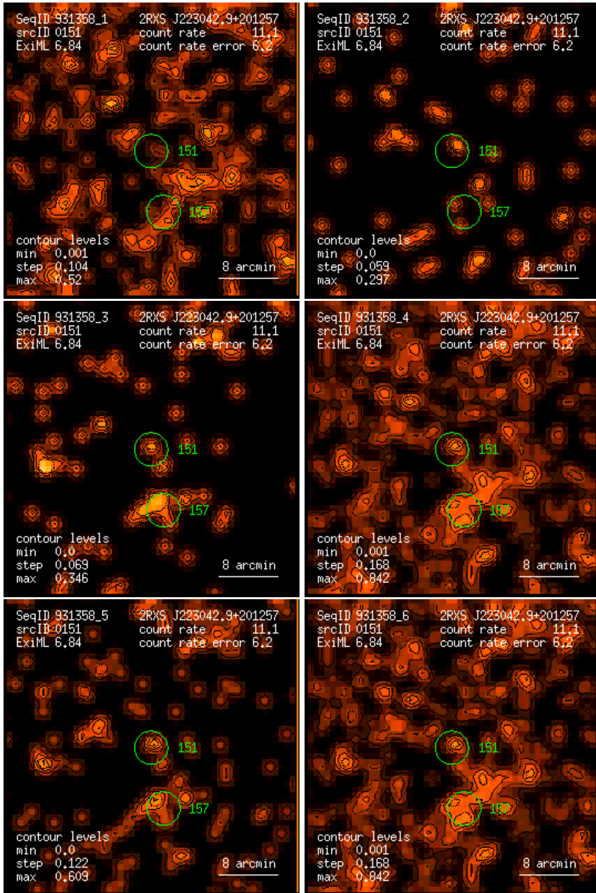
Figure 151: RASS 931358: detection 0151: band rate images, Gaussian filter: (1) PSPC channels 11 – 41, (2) 52 – 90, (3) 91 – 201, (4) 11 – 235, (5) 52 – 201, (6) 11 – 201. Broad band rates in counts/ks. Band rate contour levels in counts/ks/arcmin 2 .
