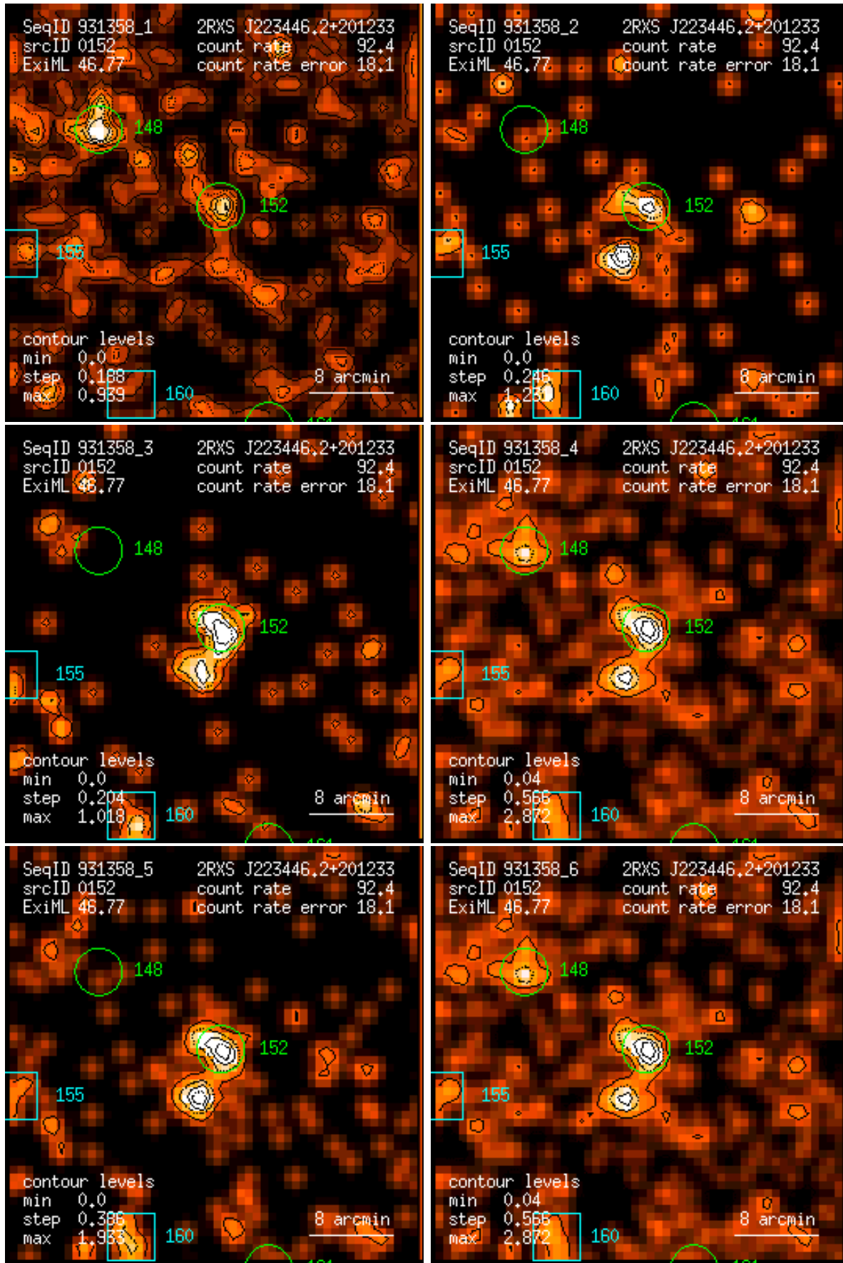
Figure 152: RASS 931358: detection 0152: band rate images, Gaussian filter: (1) PSPC channels 11 – 41, (2) 52 – 90, (3) 91 – 201, (4) 11 – 235, (5) 52 – 201, (6) 11 – 201. Broad band rates in counts/ks. Band rate contour levels in counts/ks/arcmin 2 .
