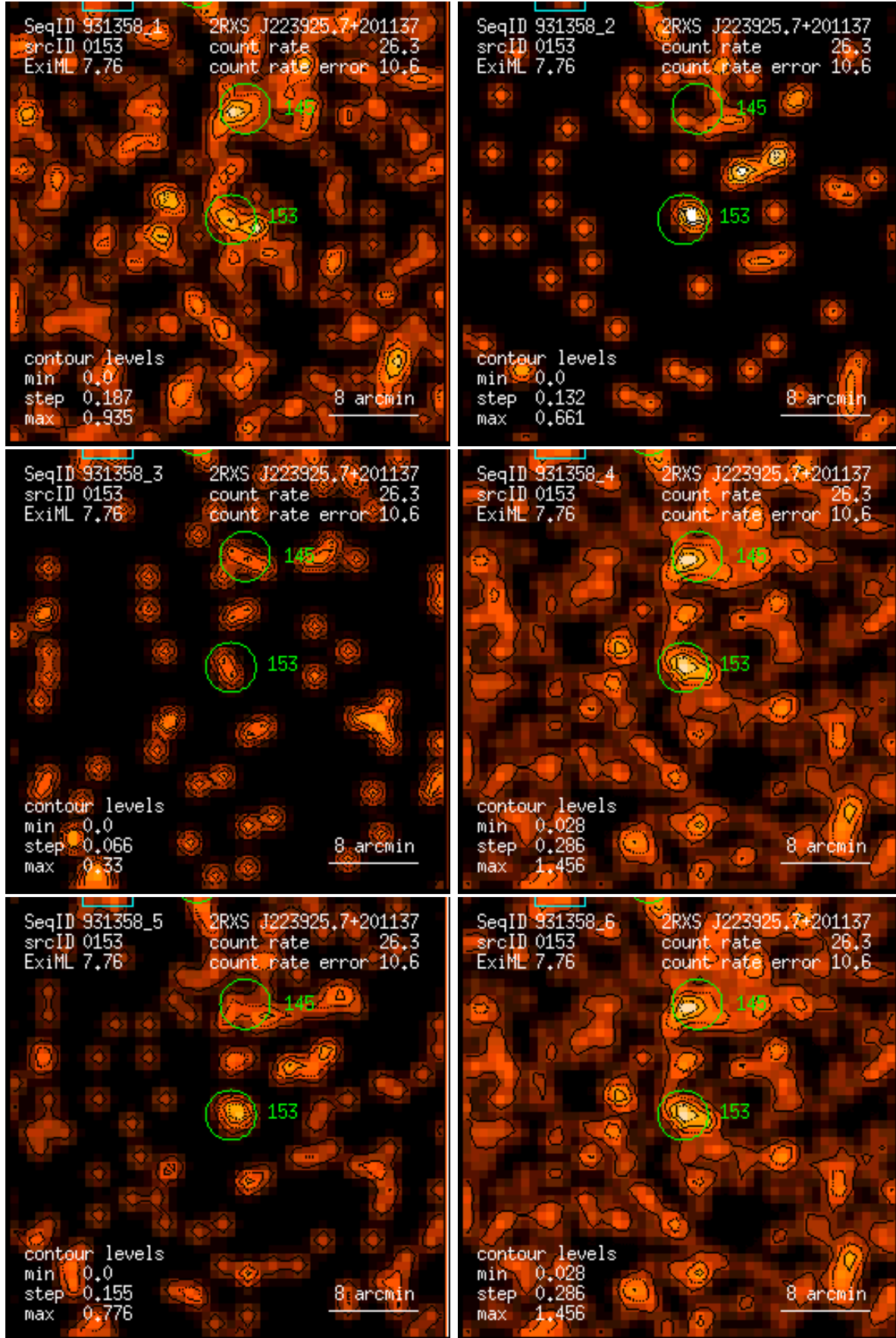
Figure 153: RASS 931358: detection 0153: band rate images, Gaussian filter: (1) PSPC channels 11 – 41, (2) 52 – 90, (3) 91 – 201, (4) 11 – 235, (5) 52 – 201, (6) 11 – 201. Broad band rates in counts/ks. Band rate contour levels in counts/ks/arcmin 2 .
