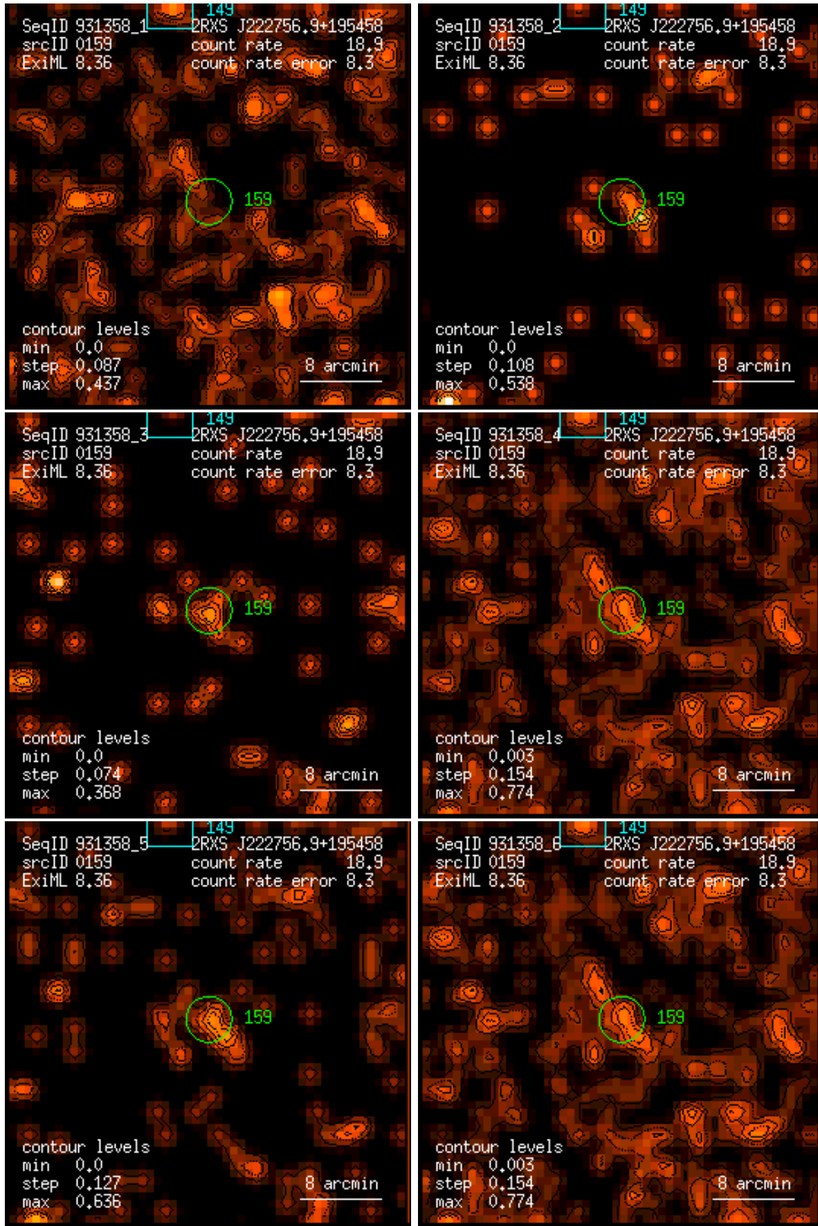
Figure 159: RASS 931358: detection 0159: band rate images, Gaussian filter: (1) PSPC channels 11 – 41, (2) 52 – 90, (3) 91 – 201, (4) 11 – 235, (5) 52 – 201, (6) 11 – 201. Broad band rates in counts/ks. Band rate contour levels in counts/ks/arcmin 2 .
