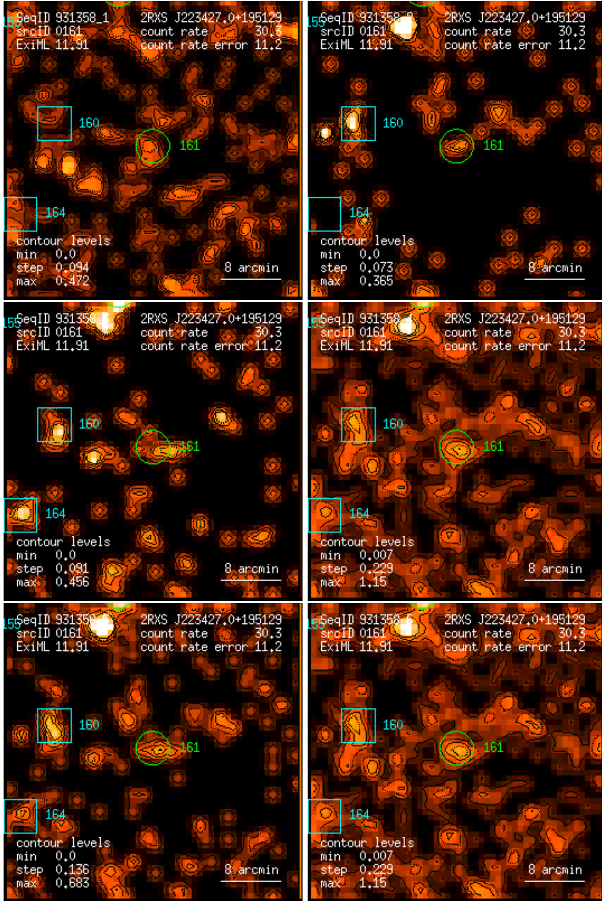
Figure 161: RASS 931358: detection 0161: band rate images, Gaussian filter: (1) PSPC channels 11 – 41, (2) 52 – 90, (3) 91 – 201, (4) 11 – 235, (5) 52 – 201, (6) 11 – 201. Broad band rates in counts/ks. Band rate contour levels in counts/ks/arcmin 2 .
