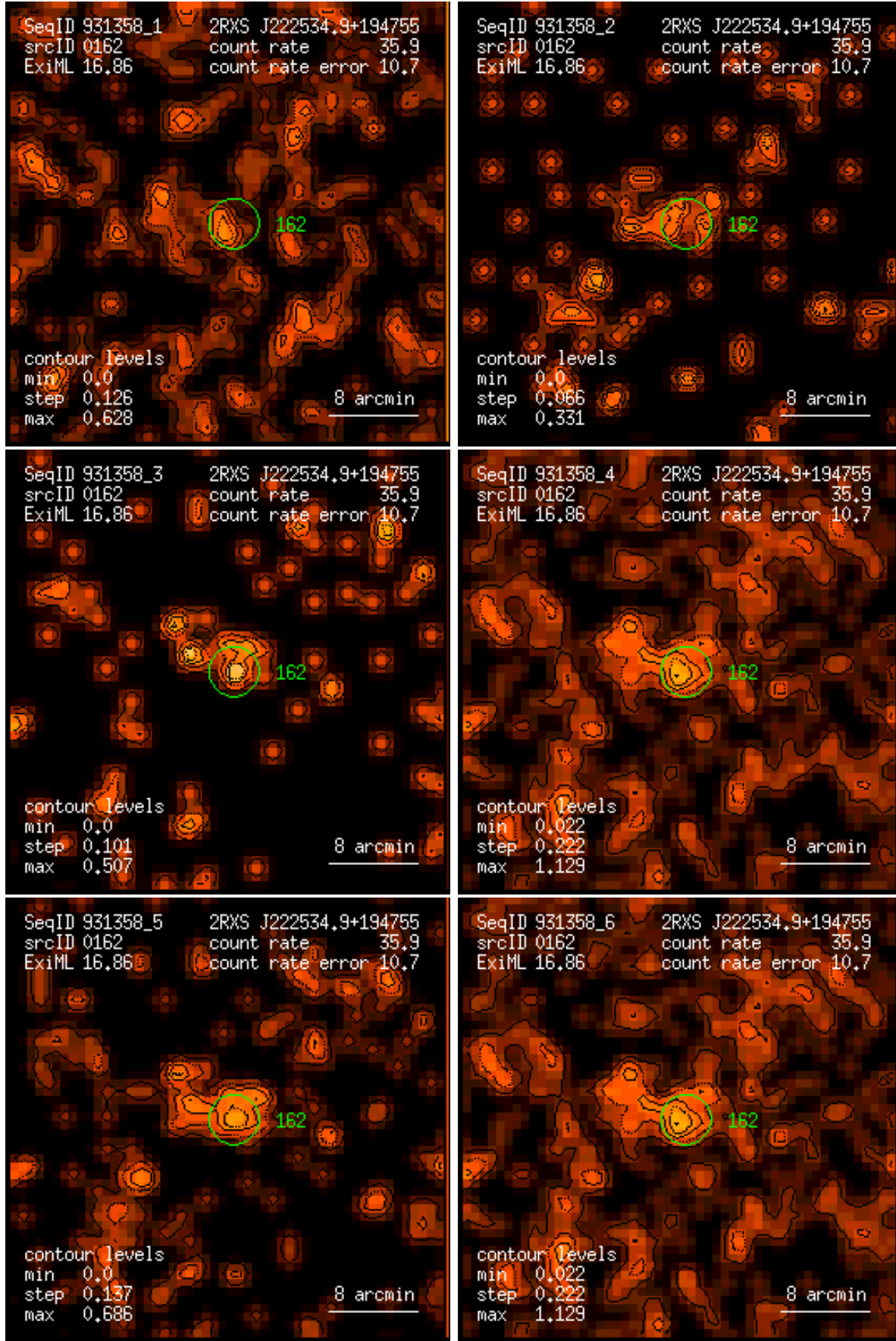
Figure 162: RASS 931358: detection 0162: band rate images, Gaussian filter: (1) PSPC channels 11 – 41, (2) 52 – 90, (3) 91 – 201, (4) 11 – 235, (5) 52 – 201, (6) 11 – 201. Broad band rates in counts/ks. Band rate contour levels in counts/ks/arcmin 2 .
