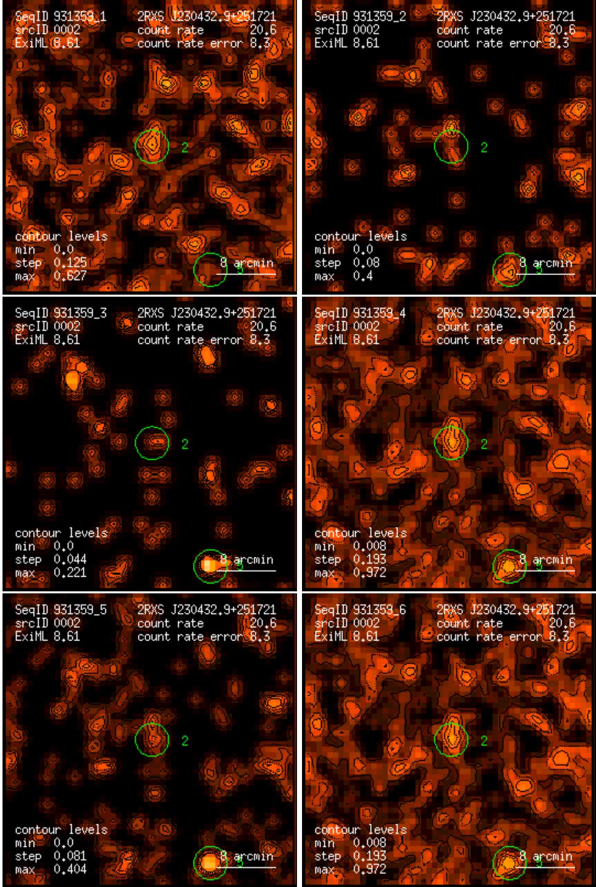
Figure 2: RASS 931359: detection 0002: band rate images, Gaussian filter: (1) PSPC channels 11 – 41, (2) 52 – 90, (3) 91 – 201, (4) 11 – 235, (5) 52 – 201, (6) 11 – 201. Broad band rates in counts/ks. Band rate contour levels in counts/ks/arcmin 2 .
