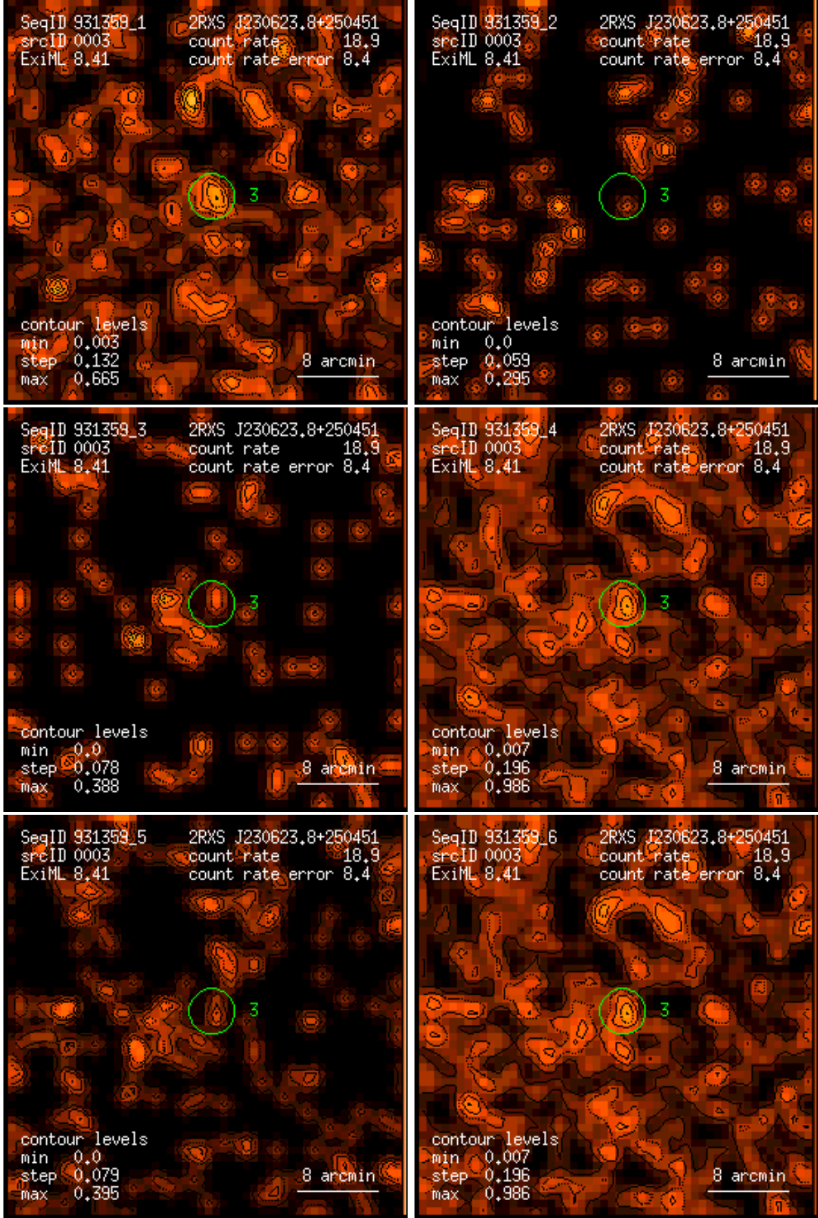
Figure 3: RASS 931359: detection 0003: band rate images, Gaussian filter: (1) PSPC channels 11 – 41, (2) 52 – 90, (3) 91 – 201, (4) 11 – 235, (5) 52 – 201, (6) 11 – 201. Broad band rates in counts/ks. Band rate contour levels in counts/ks/arcmin 2 .
