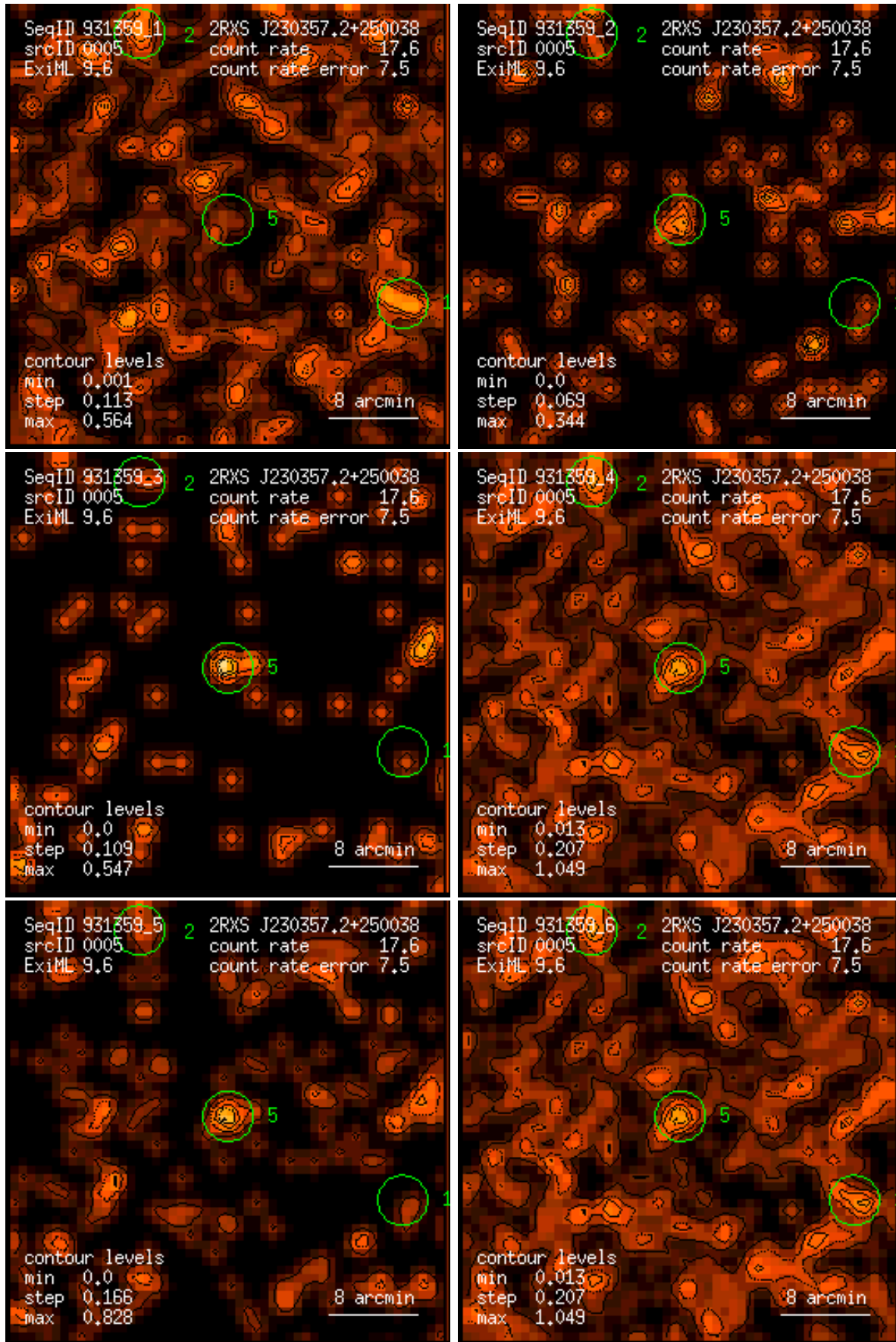
Figure 5: RASS 931359: detection 0005: band rate images, Gaussian filter: (1) PSPC channels 11 – 41, (2) 52 – 90, (3) 91 – 201, (4) 11 – 235, (5) 52 – 201, (6) 11 – 201. Broad band rates in counts/ks. Band rate contour levels in counts/ks/arcmin 2 .
