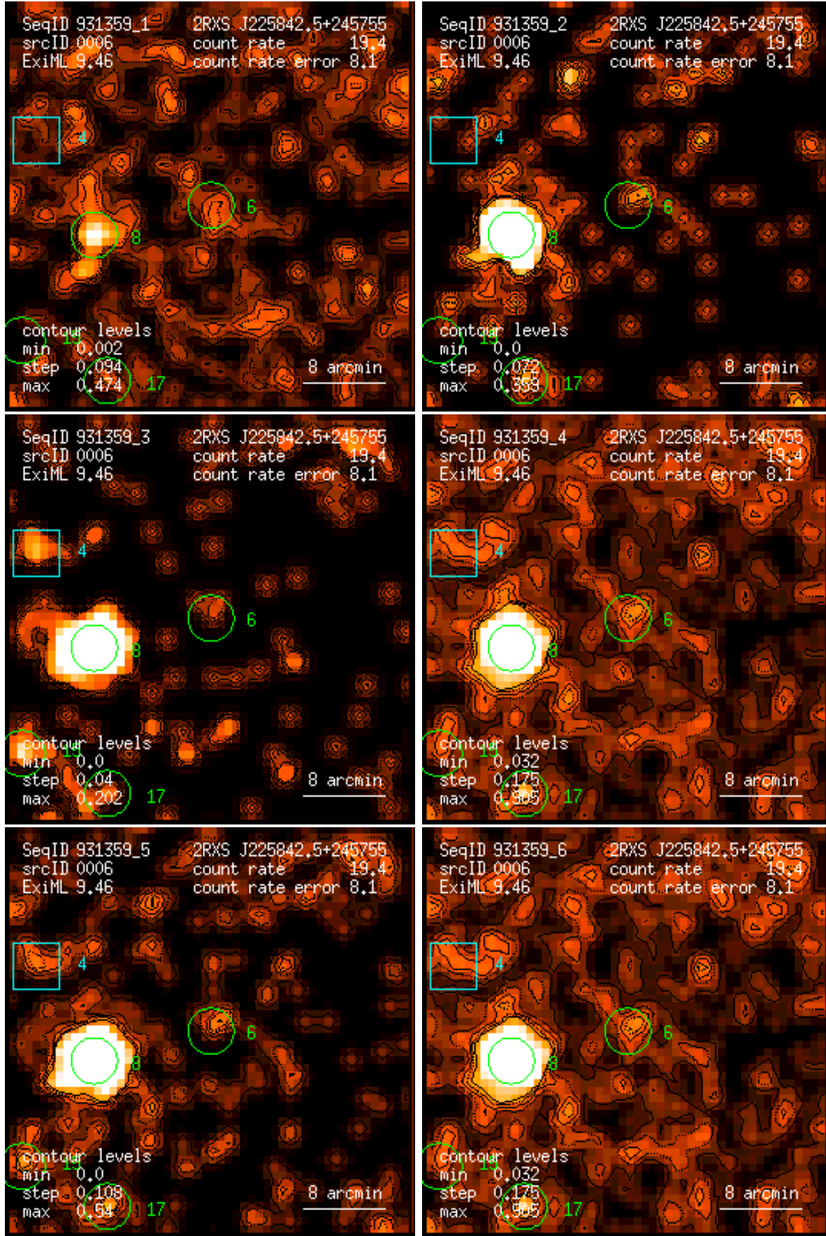
Figure 6: RASS 931359: detection 0006: band rate images, Gaussian filter: (1) PSPC channels 11 – 41, (2) 52 – 90, (3) 91 – 201, (4) 11 – 235, (5) 52 – 201, (6) 11 – 201. Broad band rates in counts/ks. Band rate contour levels in counts/ks/arcmin 2 .
