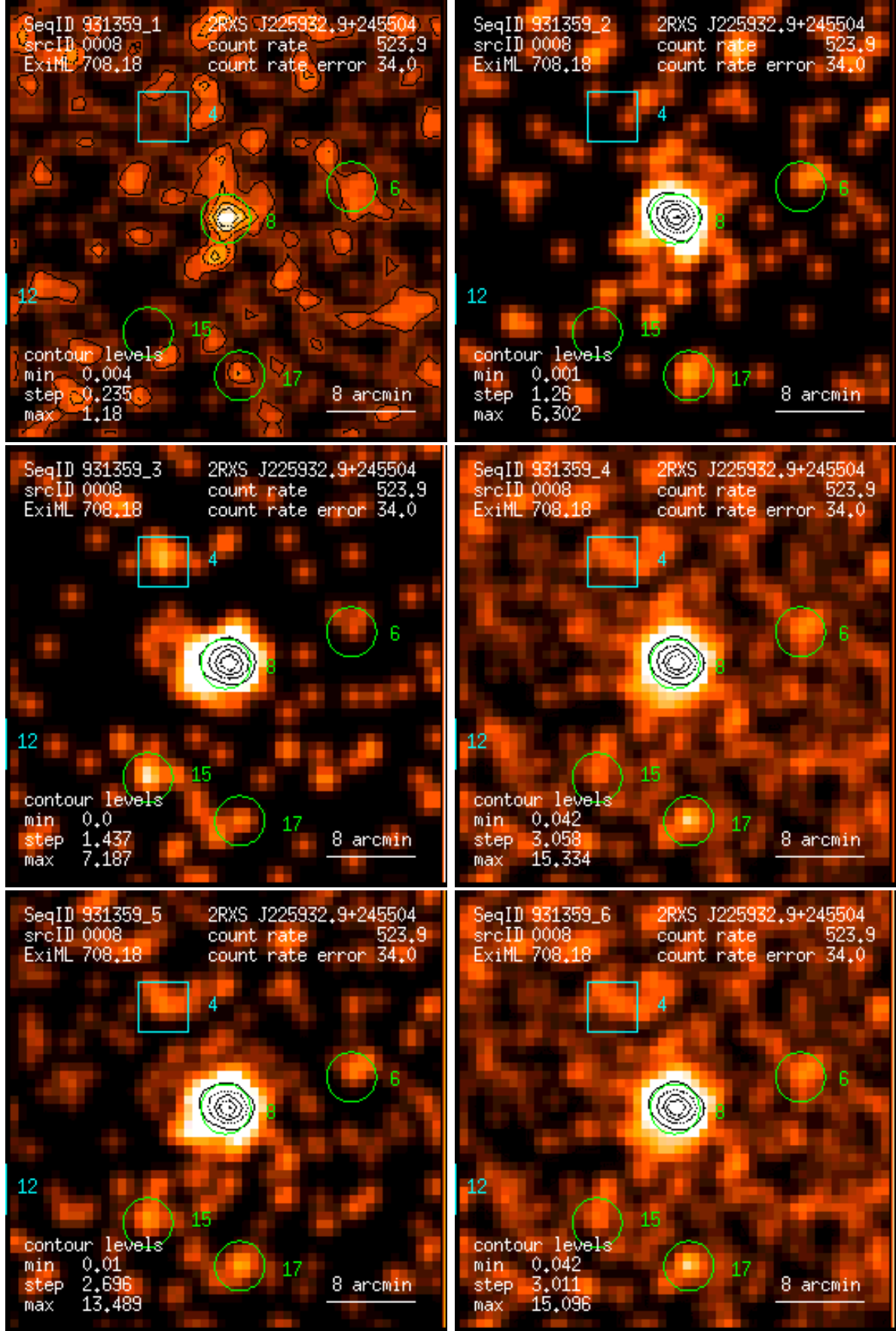
Figure 8: RASS 931359: detection 0008: band rate images, Gaussian filter: (1) PSPC channels 11 – 41, (2) 52 – 90, (3) 91 – 201, (4) 11 – 235, (5) 52 – 201, (6) 11 – 201. Broad band rates in counts/ks. Band rate contour levels in counts/ks/arcmin 2 .
