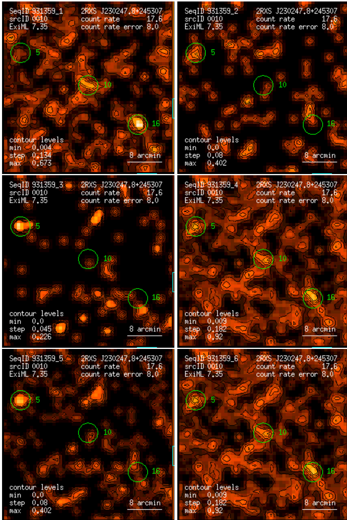
Figure 10: RASS 931359: detection 0010: band rate images, Gaussian filter: (1) PSPC channels 11 – 41, (2) 52 – 90, (3) 91 – 201, (4) 11 – 235, (5) 52 – 201, (6) 11 – 201. Broad band rates in counts/ks. Band rate contour levels in counts/ks/arcmin 2 .
