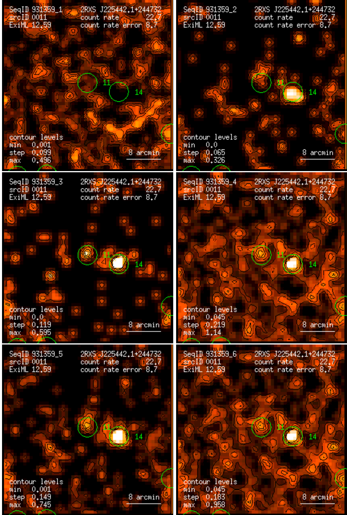
Figure 11: RASS 931359: detection 0011: band rate images, Gaussian filter: (1) PSPC channels 11 – 41, (2) 52 – 90, (3) 91 – 201, (4) 11 – 235, (5) 52 – 201, (6) 11 – 201. Broad band rates in counts/ks. Band rate contour levels in counts/ks/arcmin 2 .
