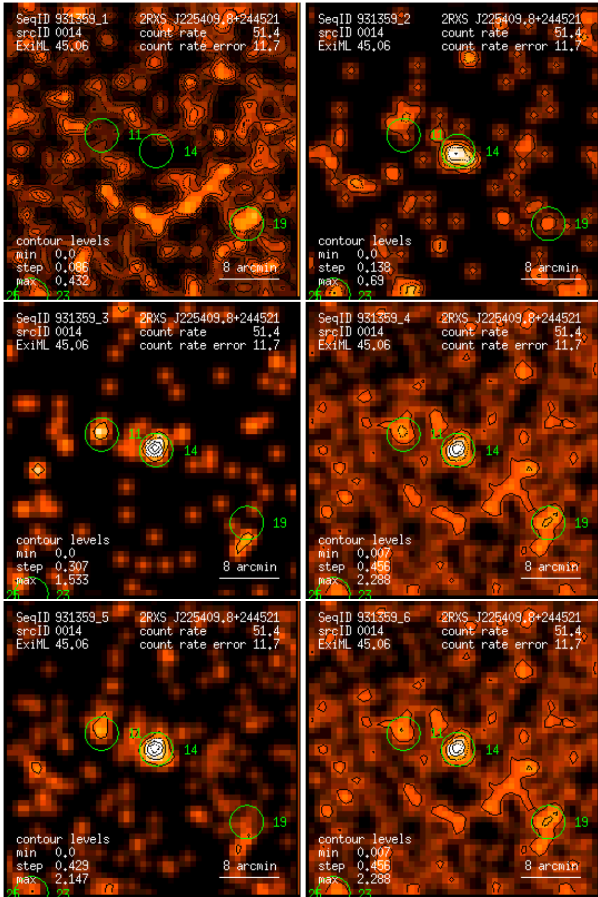
Figure 14: RASS 931359: detection 0014: band rate images, Gaussian filter: (1) PSPC channels 11 – 41, (2) 52 – 90, (3) 91 – 201, (4) 11 – 235, (5) 52 – 201, (6) 11 – 201. Broad band rates in counts/ks. Band rate contour levels in counts/ks/arcmin 2 .
