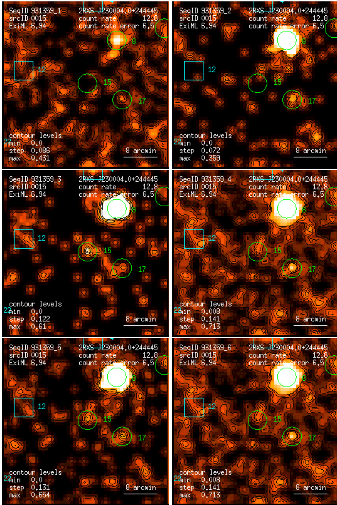
Figure 15: RASS 931359: detection 0015: band rate images, Gaussian filter: (1) PSPC channels 11 – 41, (2) 52 – 90, (3) 91 – 201, (4) 11 – 235, (5) 52 – 201, (6) 11 – 201. Broad band rates in counts/ks. Band rate contour levels in counts/ks/arcmin 2 .
