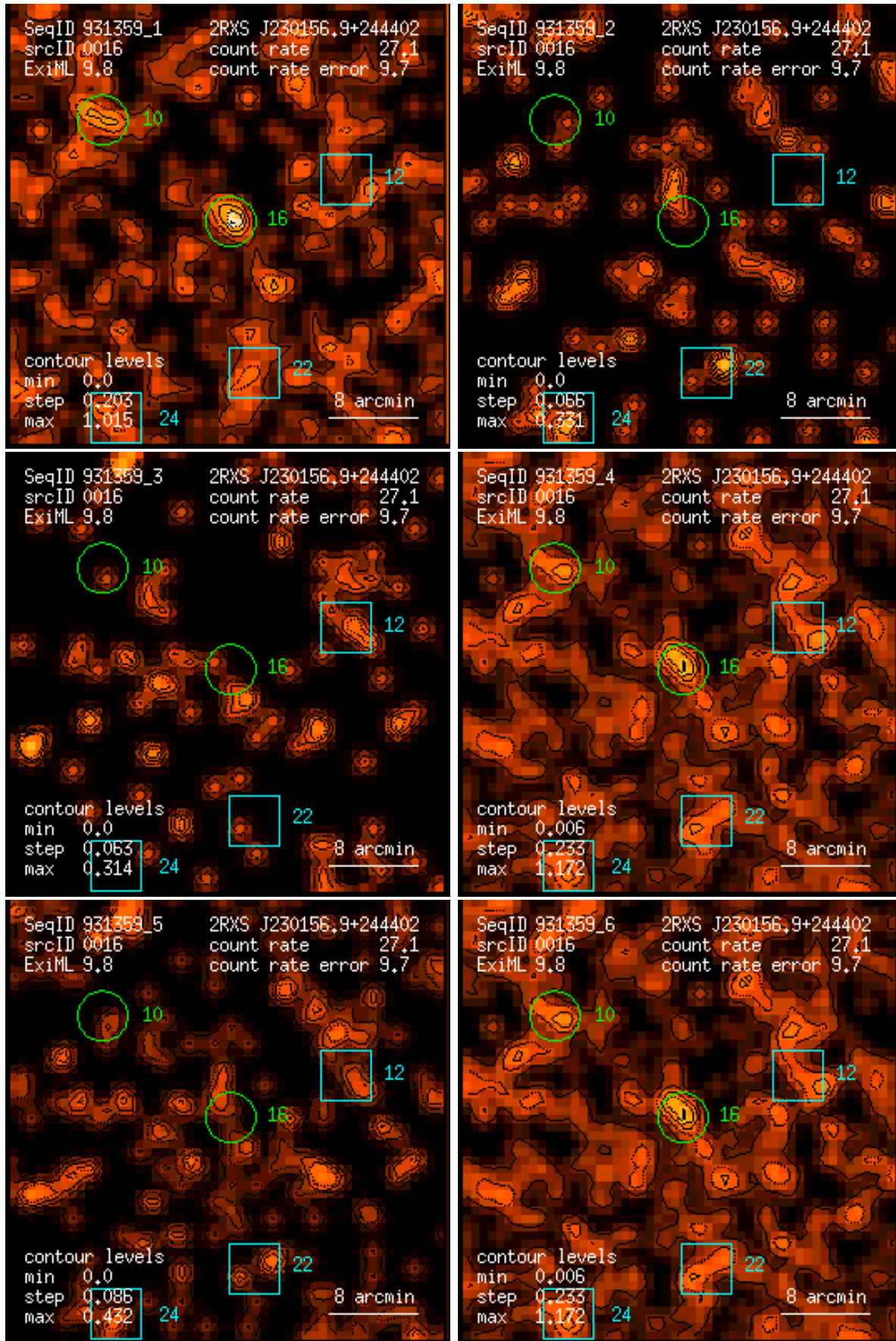
Figure 16: RASS 931359: detection 0016: band rate images, Gaussian filter: (1) PSPC channels 11 – 41, (2) 52 – 90, (3) 91 – 201, (4) 11 – 235, (5) 52 – 201, (6) 11 – 201. Broad band rates in counts/ks. Band rate contour levels in counts/ks/arcmin 2 .
