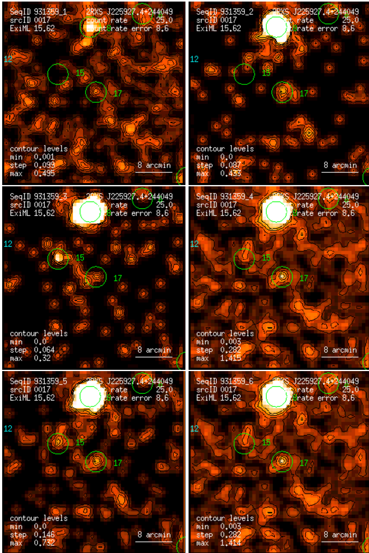
Figure 17: RASS 931359: detection 0017: band rate images, Gaussian filter: (1) PSPPC channels 11 – 41, (2) 52 – 90, (3) 91 – 201, (4) 11 – 235, (5) 52 – 201, (6) 11 – 201. Broad band rates in counts/ks. Band rate contour levels in counts/ks/arcmin 2 .
