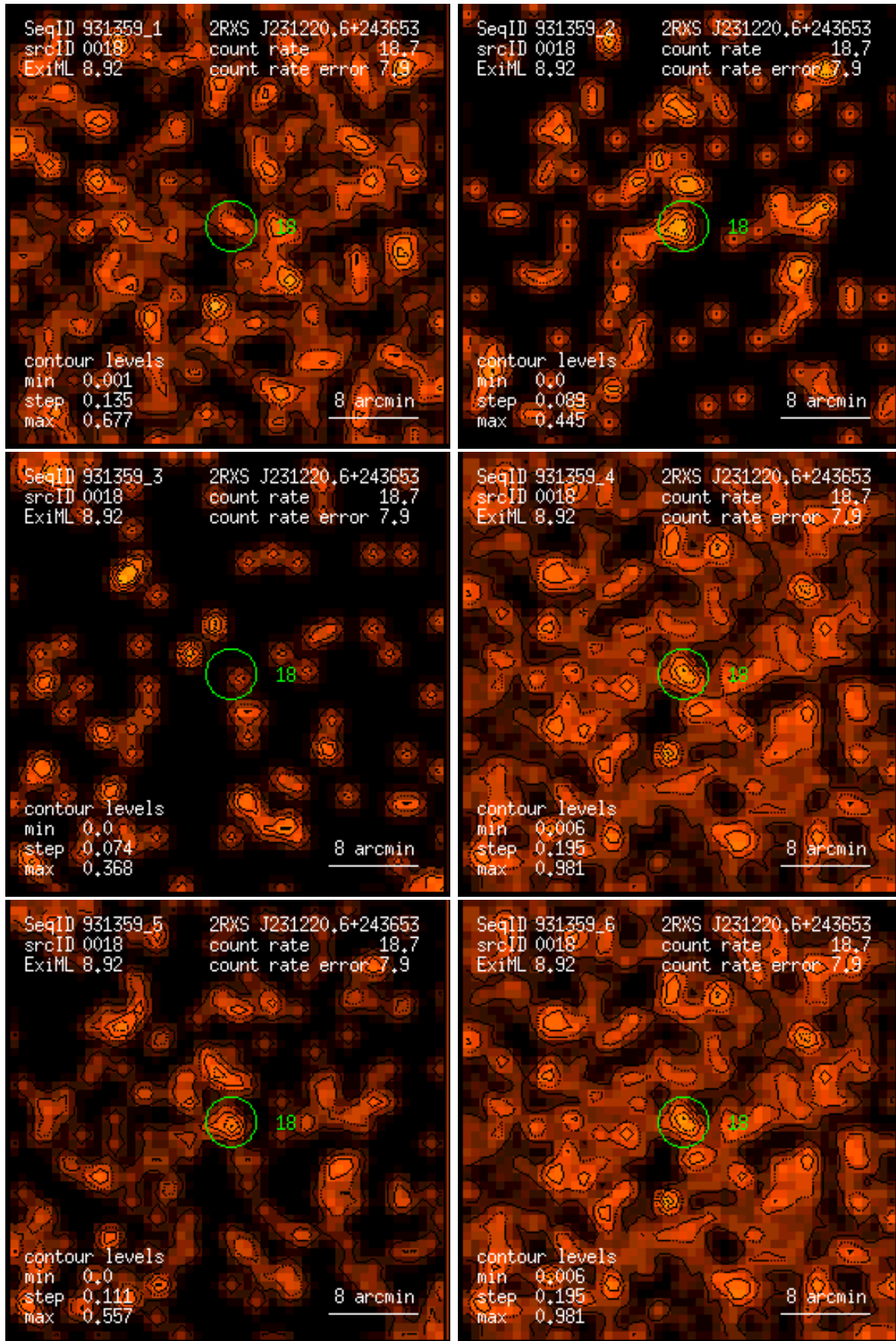
Figure 18: RASS 931359: detection 0018: band rate images, Gaussian filter: (1) PSPC channels 11 – 41, (2) 52 – 90, (3) 91 – 201, (4) 11 – 235, (5) 52 – 201, (6) 11 – 201. Broad band rates in counts/ks. Band rate contour levels in counts/ks/arcmin 2 .
