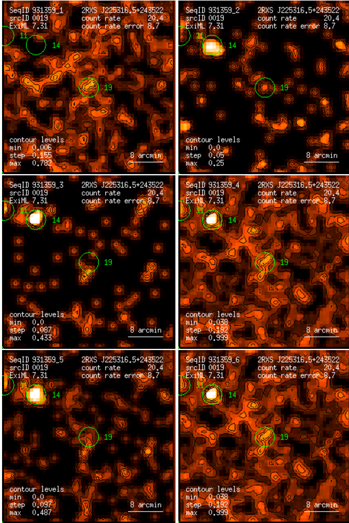
Figure 19: RASS 931359: detection 0019: band rate images, Gaussian filter: (1) PSPC channels 11 – 41, (2) 52 – 90, (3) 91 – 201, (4) 11 – 235, (5) 52 – 201, (6) 11 – 201. Broad band rates in counts/ks. Band rate contour levels in counts/ks/arcmin 2 .
