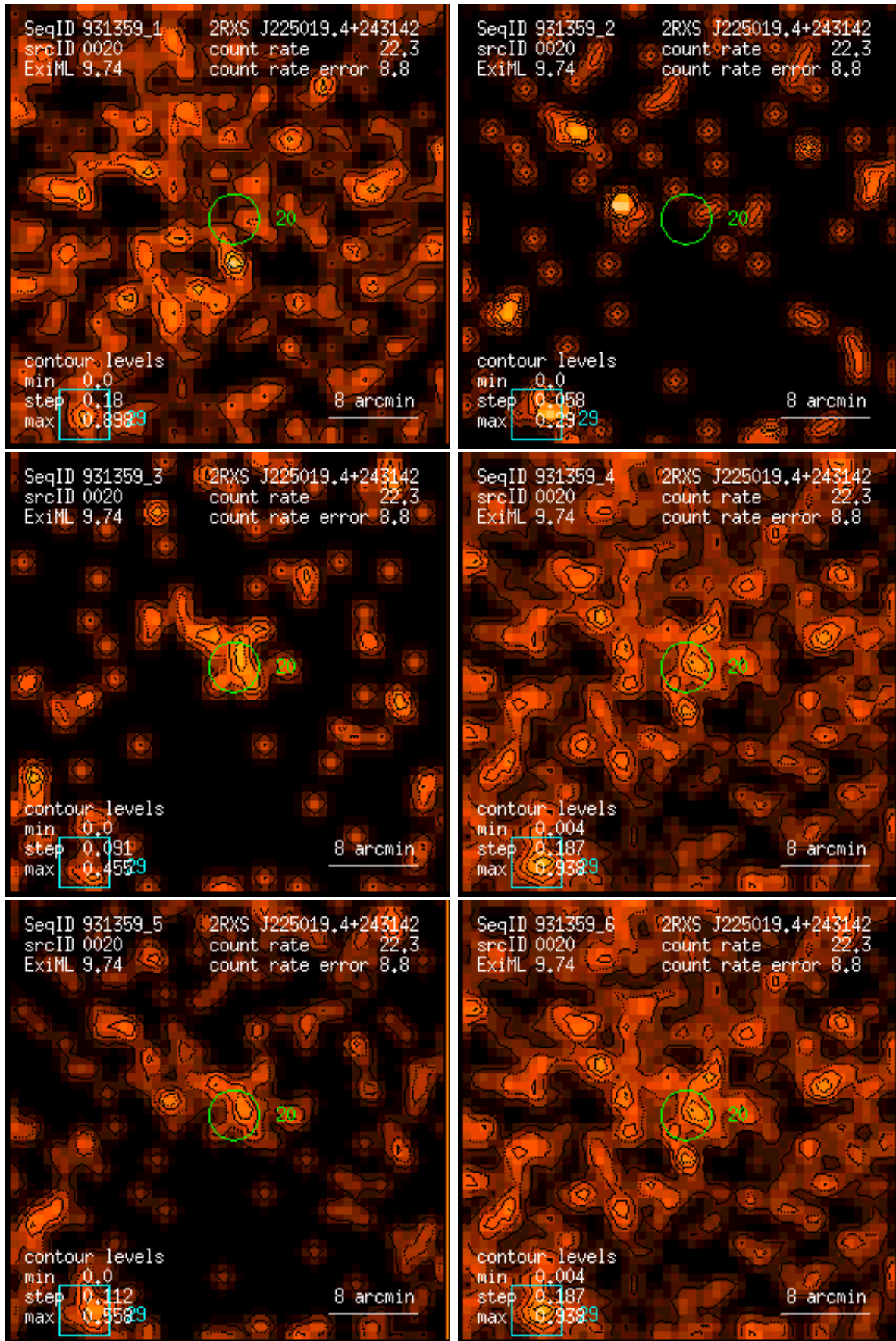
Figure 20: RASS 931359: detection 0020: band rate images, Gaussian filter: (1) PSPC channels 11 – 41, (2) 52 – 90, (3) 91 – 201, (4) 11 – 235, (5) 52 – 201, (6) 11 – 201. Broad band rates in counts/ks. Band rate contour levels in counts/ks/arcmin 2 .
