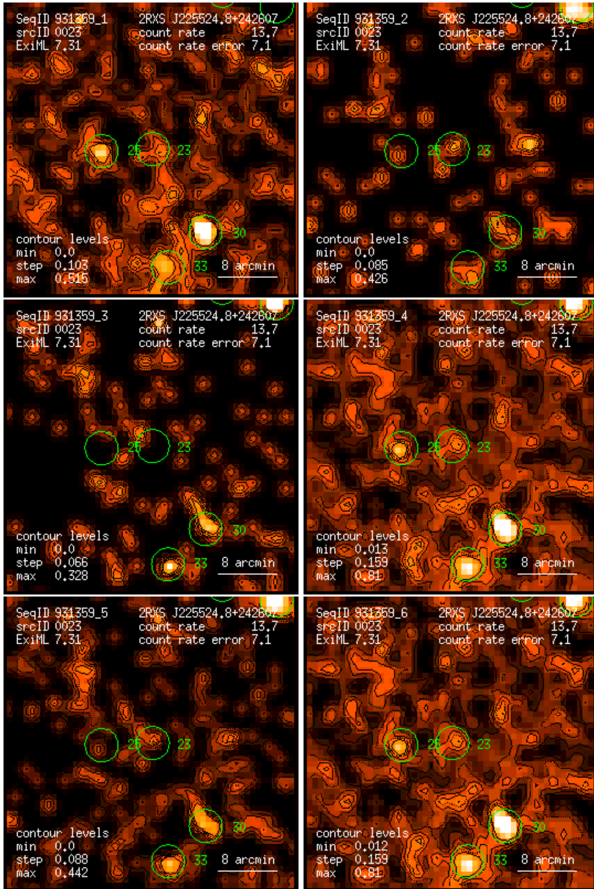
Figure 23: RASS 931359: detection 0023: band rate images, Gaussian filter: (1) PSPC channels 11 – 41, (2) 52 – 90, (3) 91 – 201, (4) 11 – 235, (5) 52 – 201, (6) 11 – 201. Broad band rates in counts/ks. Band rate contour levels in counts/ks/arcmin 2 .
