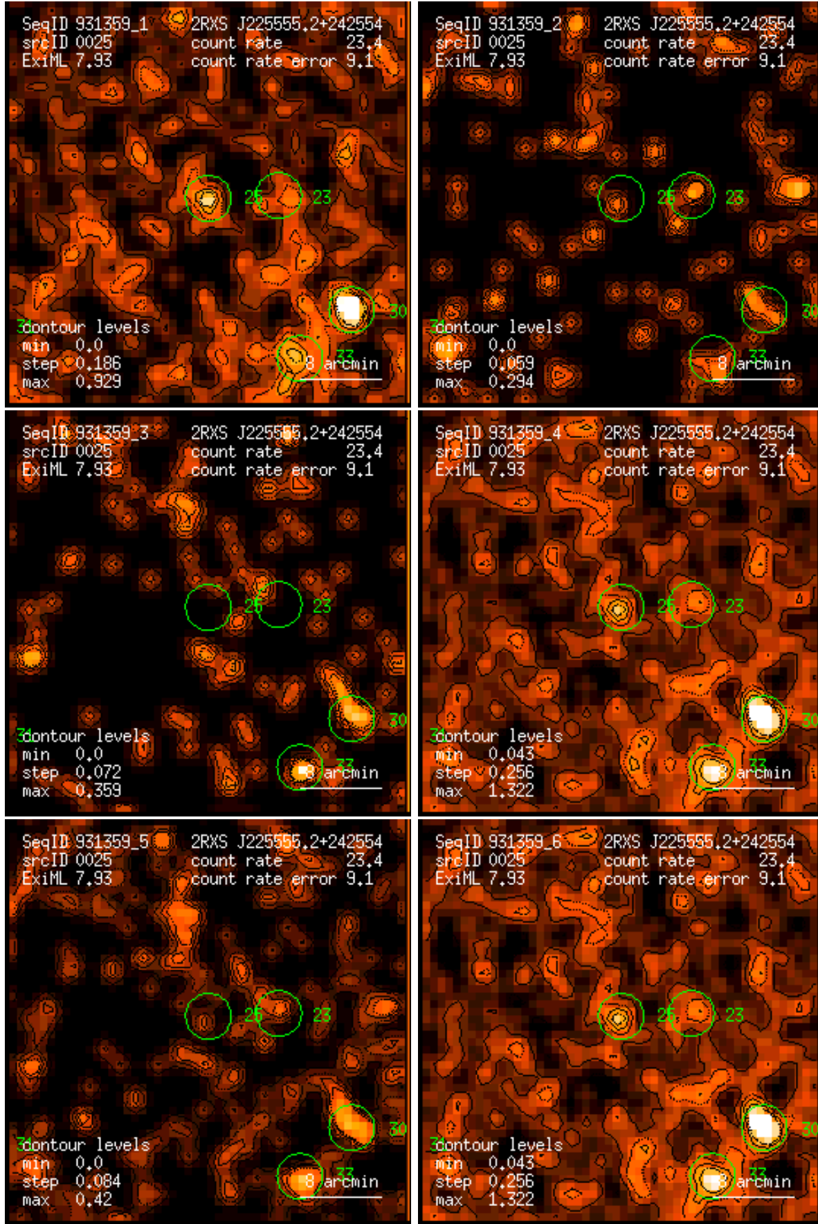
Figure 25: RASS 931359: detection 0025: band rate images, Gaussian filter: (1) PSPC channels 11 – 41, (2) 52 – 90, (3) 91 – 201, (4) 11 – 235, (5) 52 – 201, (6) 11 – 201. Broad band rates in counts/ks. Band rate contour levels in counts/ks/arcmin 2 .
