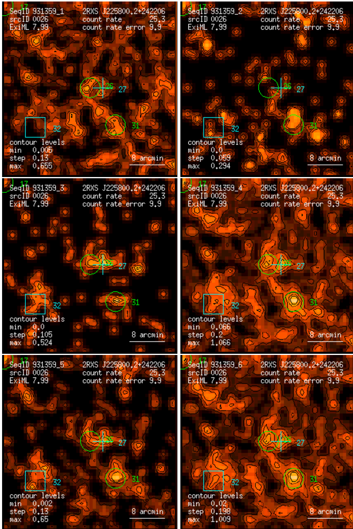
Figure 26: RASS 931359: detection 0026: band rate images, Gaussian filter: (1) PSPC channels 11 – 41, (2) 52 – 90, (3) 91 – 201, (4) 11 – 235, (5) 52 – 201, (6) 11 – 201. Broad band rates in counts/ks. Band rate contour levels in counts/ks/arcmin 2 .
