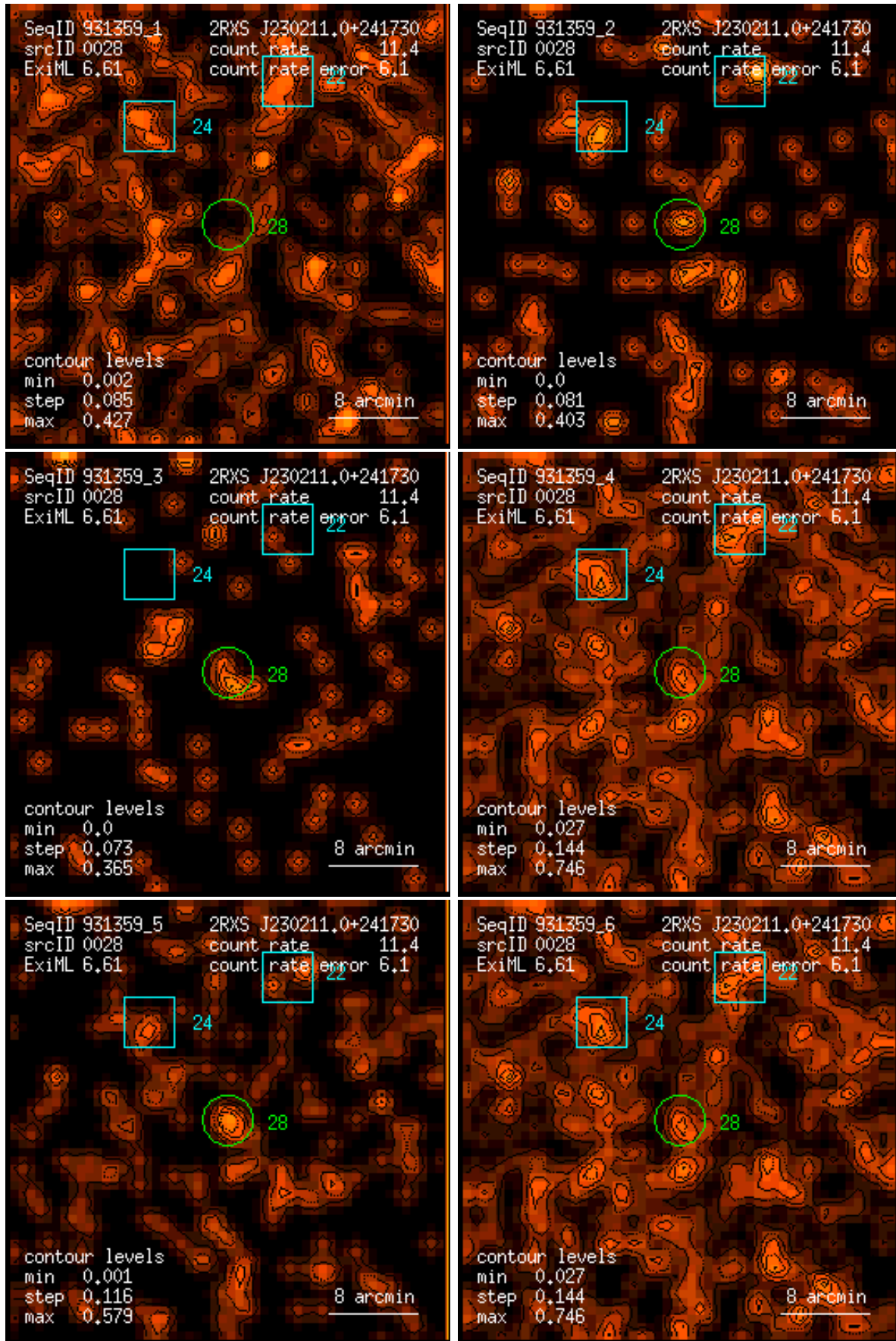
Figure 28: RASS 931359: detection 0028: band rate images, Gaussian filter: (1) PSPC channels 11 – 41, (2) 52 – 90, (3) 91 – 201, (4) 11 – 235, (5) 52 – 201, (6) 11 – 201. Broad band rates in counts/ks. Band rate contour levels in counts/ks/arcmin 2 .
