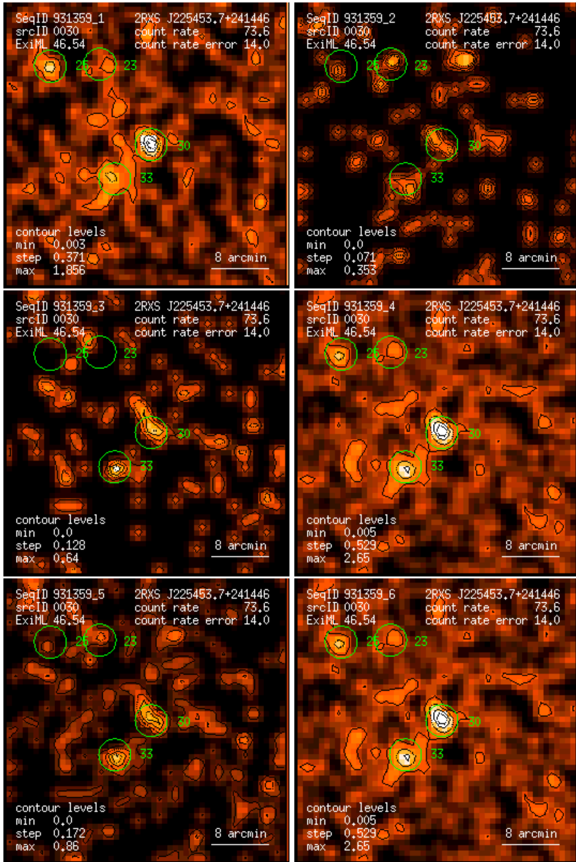
Figure 30: RASS 931359: detection 0030: band rate images, Gaussian filter: (1) PSPC channels 11 – 41, (2) 52 – 90, (3) 91 – 201, (4) 11 – 235, (5) 52 – 201, (6) 11 – 201. Broad band rates in counts/ks. Band rate contour levels in counts/ks/arcmin 2 .
