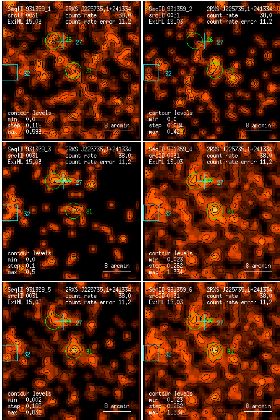
Figure 31: RASS 931359: detection 0031: band rate images, Gaussian filter: (1) PSPC channels 11 – 41, (2) 52 – 90, (3) 91 – 201, (4) 11 – 235, (5) 52 – 201, (6) 11 – 201. Broad band rates in counts/ks. Band rate contour levels in counts/ks/arcmin 2 .
