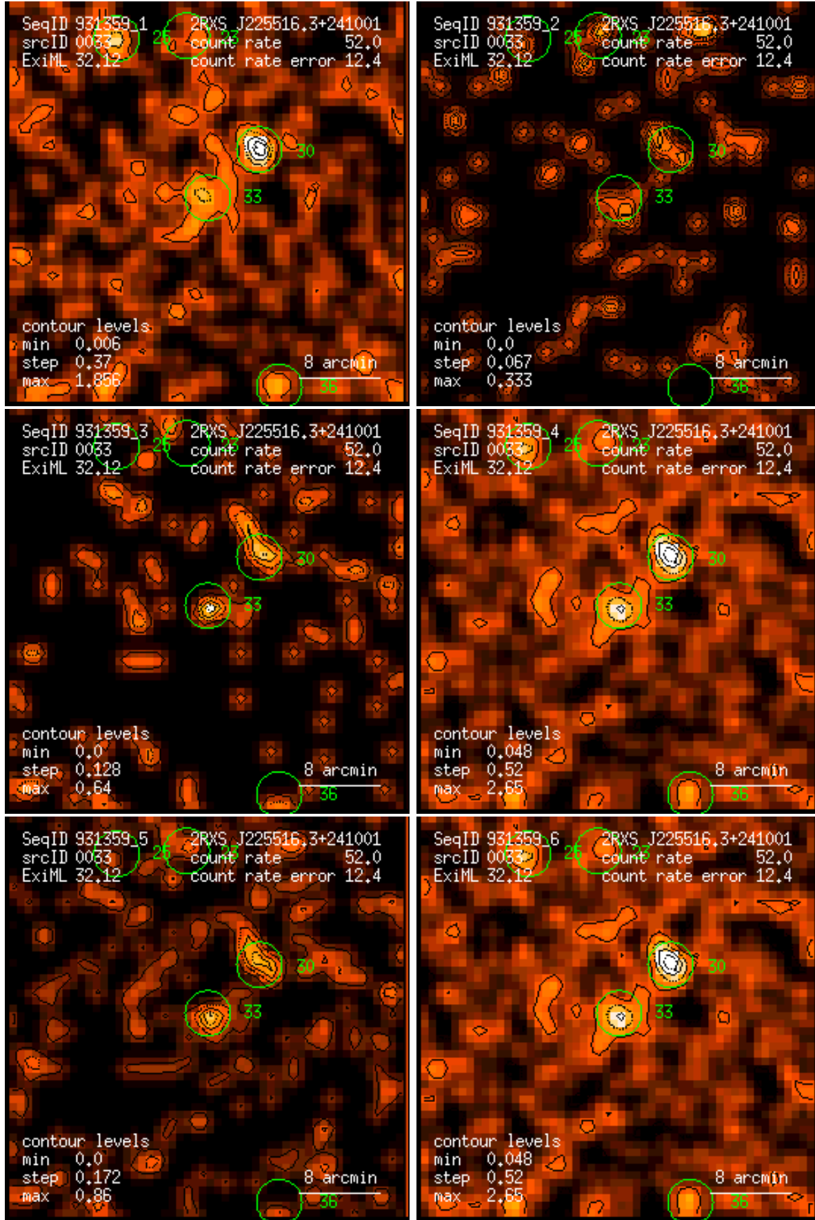
Figure 33: RASS 931359: detection 0033: band rate images, Gaussian filter: (1) PSPC channels 11 – 41, (2) 52 – 90, (3) 91 – 201, (4) 11 – 235, (5) 52 – 201, (6) 11 – 201. Broad band rates in counts/ks. Band rate contour levels in counts/ks/arcmin 2 .
