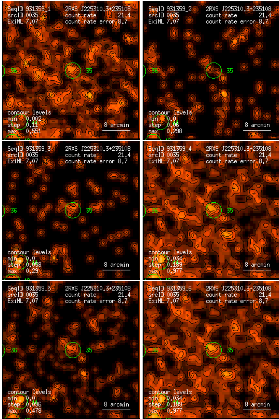
Figure 35: RASS 931359: detection 0035: band rate images, Gaussian filter: (1) PSPC channels 11 – 41, (2) 52 – 90, (3) 91 – 201, (4) 11 – 235, (5) 52 – 201, (6) 11 – 201. Broad band rates in counts/ks. Band rate contour levels in counts/ks/arcmin 2 .
