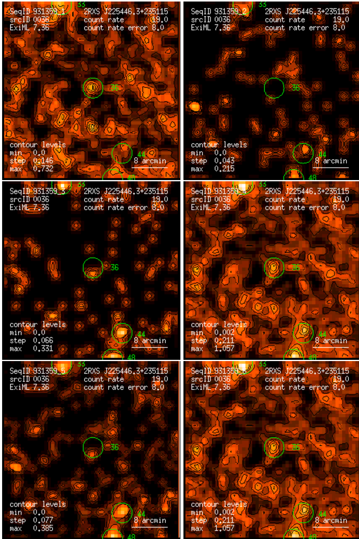
Figure 36: RASS 931359: detection 0036: band rate images, Gaussian filter: (1) PSPC channels 11 – 41, (2) 52 – 90, (3) 91 – 201, (4) 11 – 235, (5) 52 – 201, (6) 11 – 201. Broad band rates in counts/ks. Band rate contour levels in counts/ks/arcmin 2 .
