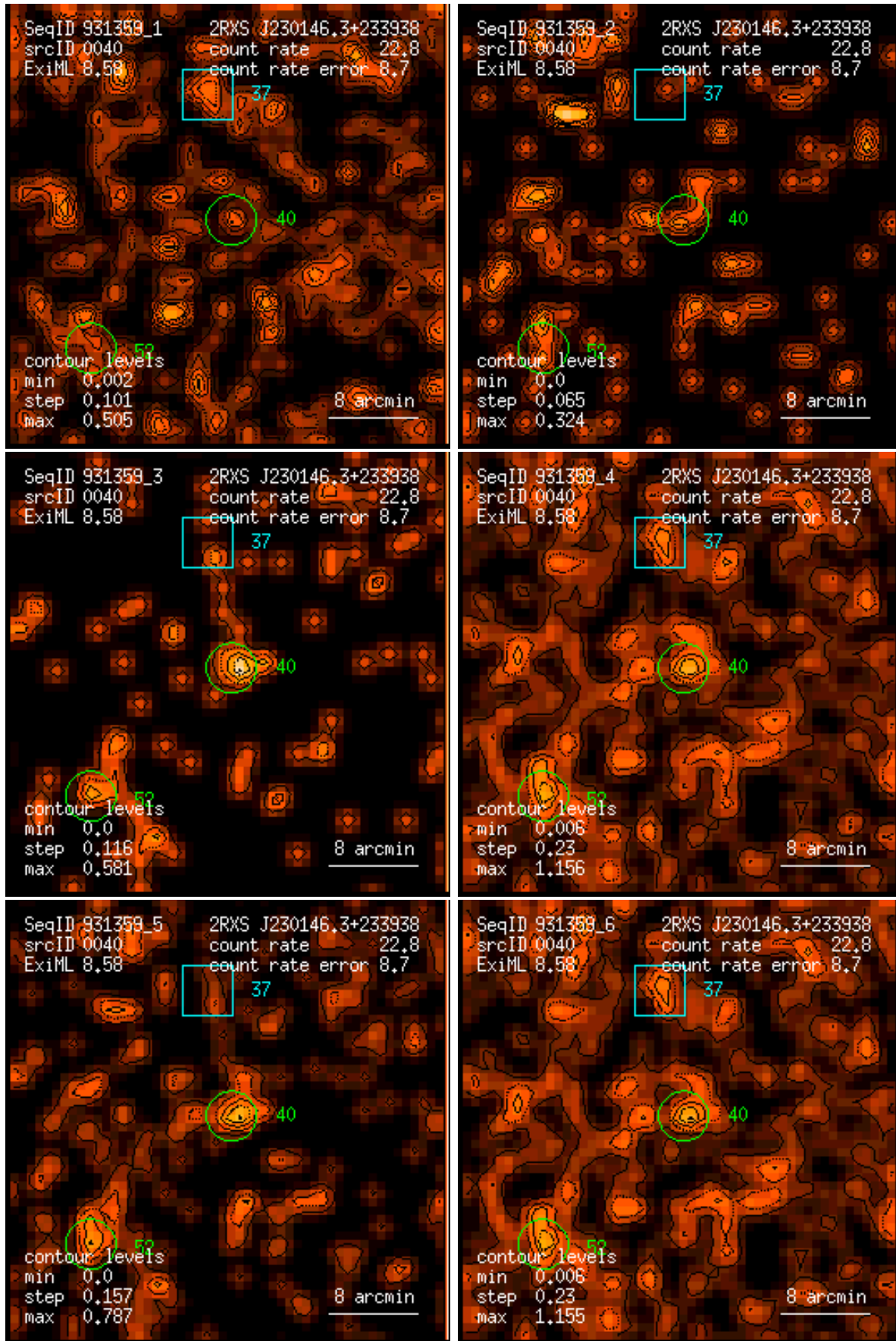
Figure 40: RASS 931359: detection 0040: band rate images, Gaussian filter: (1) PSPC channels 11 – 41, (2) 52 – 90, (3) 91 – 201, (4) 11 – 235, (5) 52 – 201, (6) 11 – 201. Broad band rates in counts/ks. Band rate contour levels in counts/ks/arcmin 2 .
