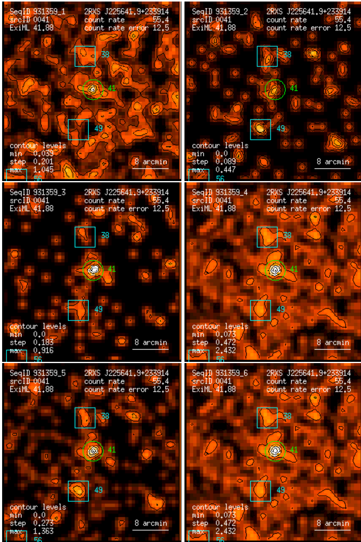
Figure 41: RASS 931359: detection 0041: band rate images, Gaussian filter: (1) PSPC channels 11 – 41, (2) 52 – 90, (3) 91 – 201, (4) 11 – 235, (5) 52 – 201, (6) 11 – 201. Broad band rates in counts/ks. Band rate contour levels in counts/ks/arcmin 2 .
