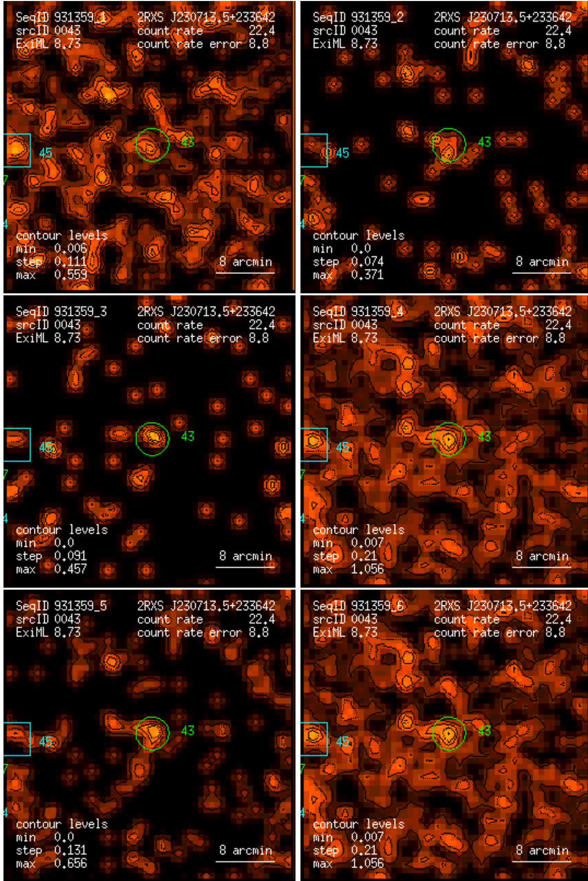
Figure 43: RASS 931359: detection 0043: band rate images, Gaussian filter: (1) PSPC channels 11 – 41, (2) 52 – 90, (3) 91 – 201, (4) 11 – 235, (5) 52 – 201, (6) 11 – 201. Broad band rates in counts/ks. Band rate contour levels in counts/ks/arcmin 2 .
